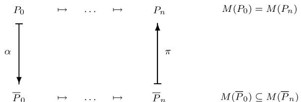
Fig. 1 Program Transformation via Well-Founded Annotations. \alpha is a well-founded annotation w.r.t. a given well-founded ordering. \pi is the projection function
