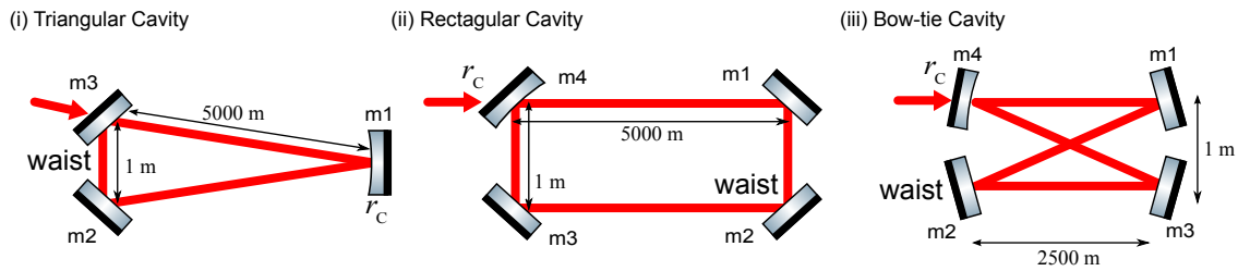
Figure 259: Cavity designs used for the numerical calculation. The cavities have a round trip length of approximately 10 km, and a beam waist at the middle point of the path.
