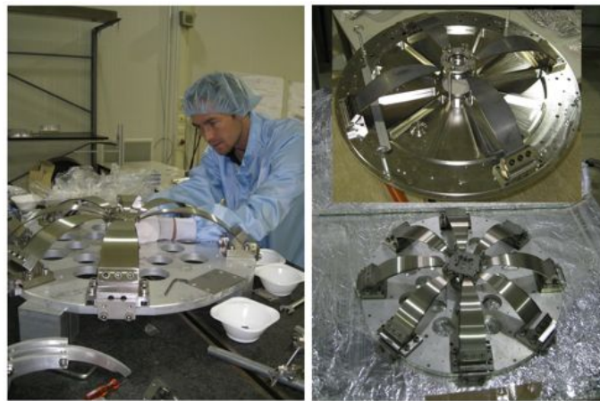
Figure 242: Pictures of the GAS filter prototypes. The left and top right panels show a filter built and tested at NIKHEF for the Virgo external injection bench [659]. The bottom right panel shows a prototype for LCGT suspension.
