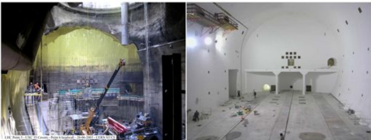
Figure 76: The construction of the CMS cavern for the LHC project at CERN, Geneva.
