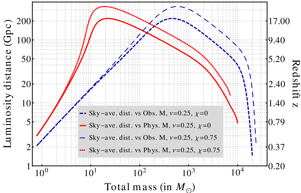
Figure 18: Distance reach of ET for signals from coalescing compact binaries, as a function of the intrinsic (red curves) and observed (blue curves) total mass. We assume that a source is visible if it produces an SNR of at least 8 in ET. Solid red and short-dashed blue curves correspond to binaries composed of non-spinning objects. Dotted red and long-dashed blue curves correspond to binaries composed of objects whose spins are aligned with the orbital angular momentum of the binary, with spin parameter \chi = 0.75 .
