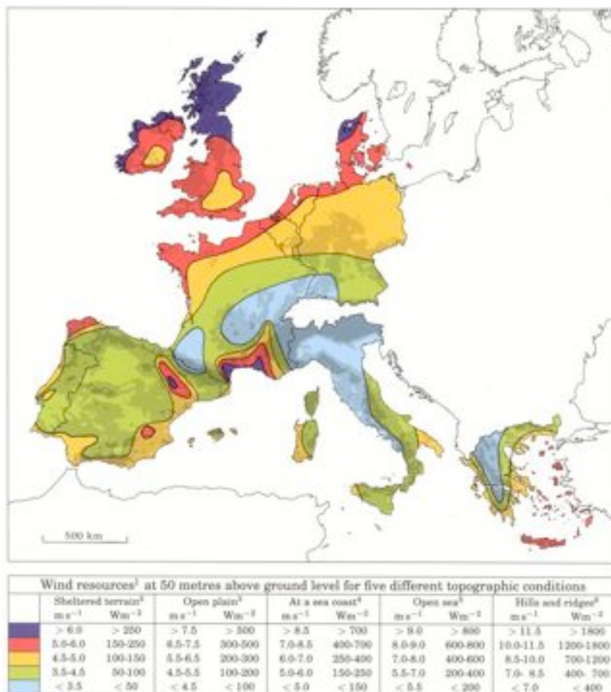
Figure 49: European wind resources based on data collected for the European Wind Atlas [294].
