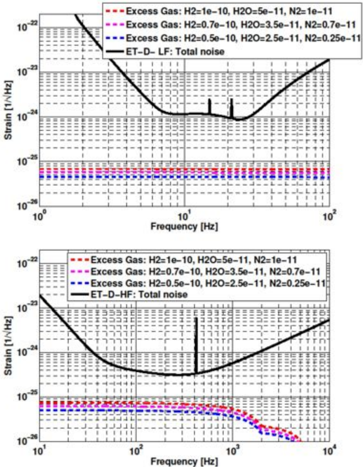
Figure 90: Phase noise given by the residual gases compared to the expected sensitivity, computed for the appropriate beam profile for different gas compositions. (Goal gas composition: Hydrogen [ 1 \cdot 10^{-10} mbar], Water [ 5 \cdot 10^{-11} mbar], Nitrogen [ 1 \cdot 10^{-11} mbar])
