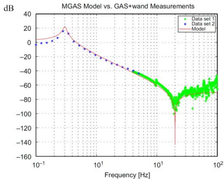
Figure 243: Vertical attenuation performance of a GAS filter with overcompensating wands [660]
