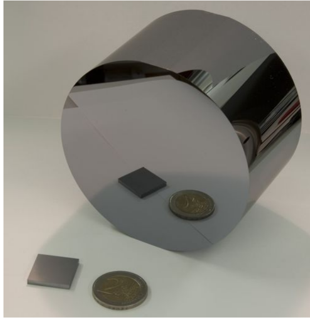
Figure 176: Silicon sample as being used for cryogenic mechanical loss measurements [380]. The single crystalline material is cut in a cylindrical shape and polished at the front and back side as well as the barrel.
