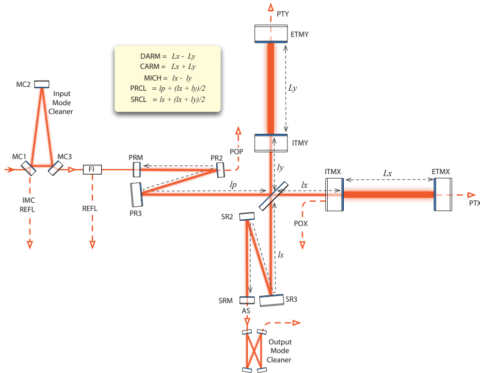
Figure 197: Schematic drawing of the Advanced LIGO optical layout, degrees-of-freedom and sensing ports [587]. Error signals for the control of the five longitudinal degrees-of-freedom are extracted from the four ports REFL, AS, POP and POX.
