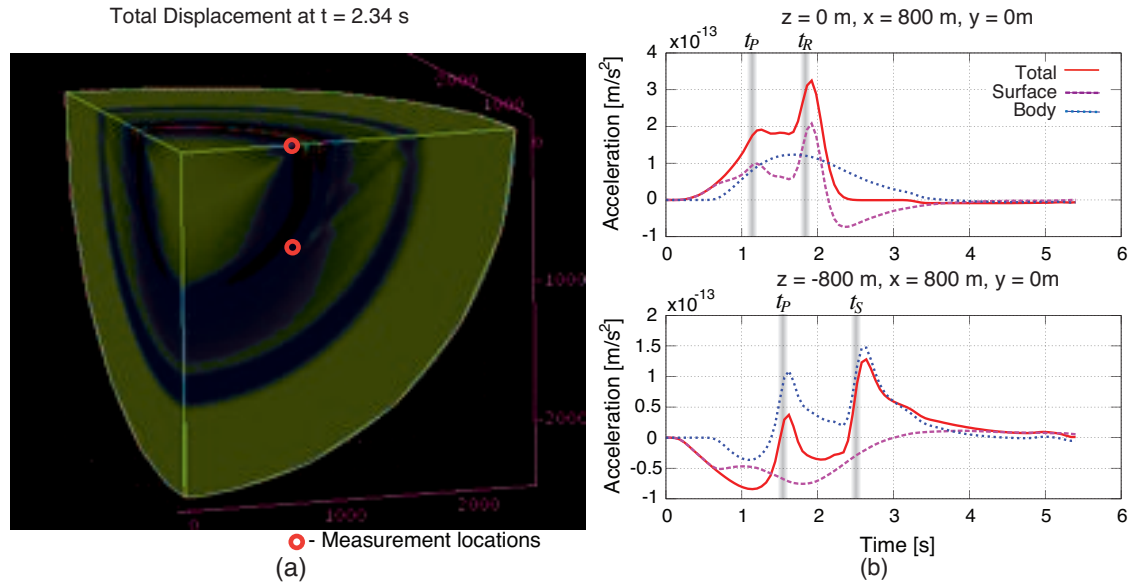
Figure 56: (a) Total displacement for a time domain simulation at 2.34 seconds after a 1 \mu\text{m} pulse excitation at the center of the half-sphere. (b) Time domain evolution of gravity gradient noise acceleration at a surface ( z=0 m) and underground ( z=-800 m, x = 800 m, y = 0 m) test mass. Only the horizontal component of the gravity gradient noise acceleration is shown. Arrival times of Rayleigh, S and P-waves are also indicated.
