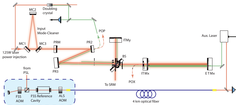
Figure 198: Schematic drawing of the Advanced LIGO arm length stabilization (ALS) subsystem [591]. The test mass motion is reduced prior to lock acquisition by a combined scheme of PDH reflection locking of an auxiliary laser to the arm cavities and heterodyne detection of the transmitted beams. The optical fiber is necessary to provide an optical reference at the end stations, to lock the auxiliary lasers' phases to the science laser.
