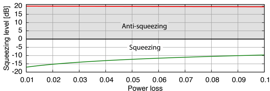
Figure 262: The degradation of the squeezing and anti-squeezing levels due to optical loss for an initially pure (no loss) 20 dB squeezed state.
