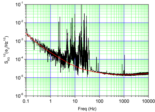
Figure 145: The magnetic flux noise spectrum produced by the SmCo magnet and referred at the SQUID loop. The spectrum is obtained by combining two spectra taken with different frequency range and averages.
