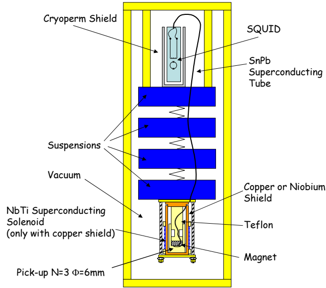
Figure 144: Experimental set for the magnetization noise measurements at 4.2 K.
