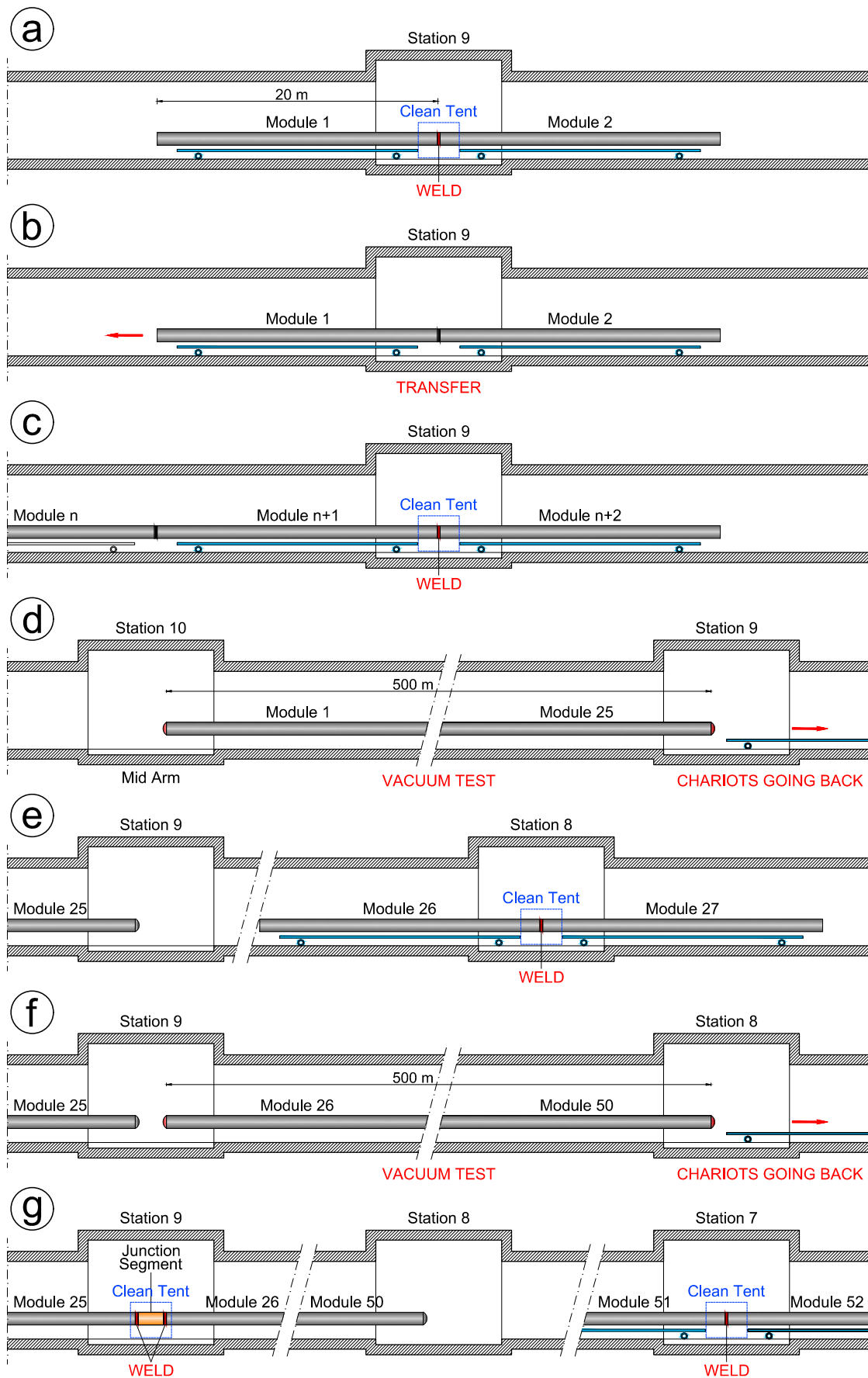
Figure 94: The assembly sequence of one vacuum pipe.
