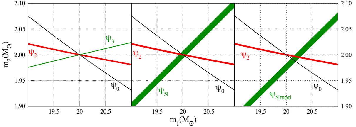
Figure 24: Curves of constant PN coefficients in the (m_1, m_2) plane for a (2, 20) M_\odot BBH merger at 300 Mpc observed in ET-B. The left and middle plots correspond to the case when the post-Newtonian coefficients are all as in GR and all three curves intersect at a single point. The plot on the right corresponds to the case when the measured value of \psi_{5l} differs from GR by 1% and in this case the three curves fail to intersect at a common point. The thickness of the lines is the 1-sigma error in the measurement of the corresponding parameter.
