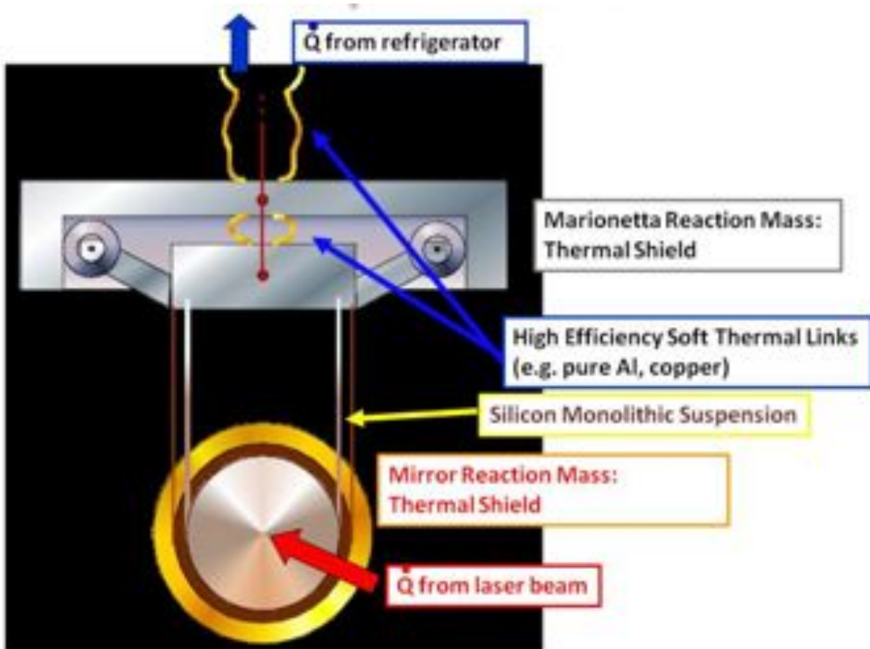
Figure 139: The conceptual scheme for a cryogenic suspension
