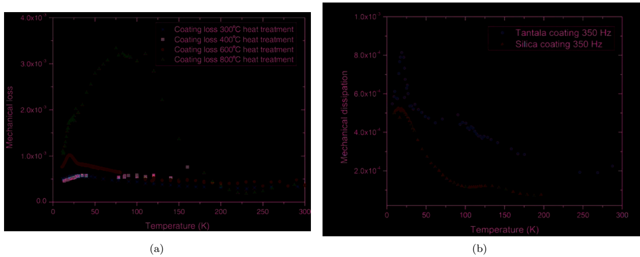
Figure 179: (a) – Measured values of the coating loss of tantala annealed at different temperatures. (b) – Comparison of 600°C heat treated tantala and silica coatings at low temperatures and 350 Hz.
