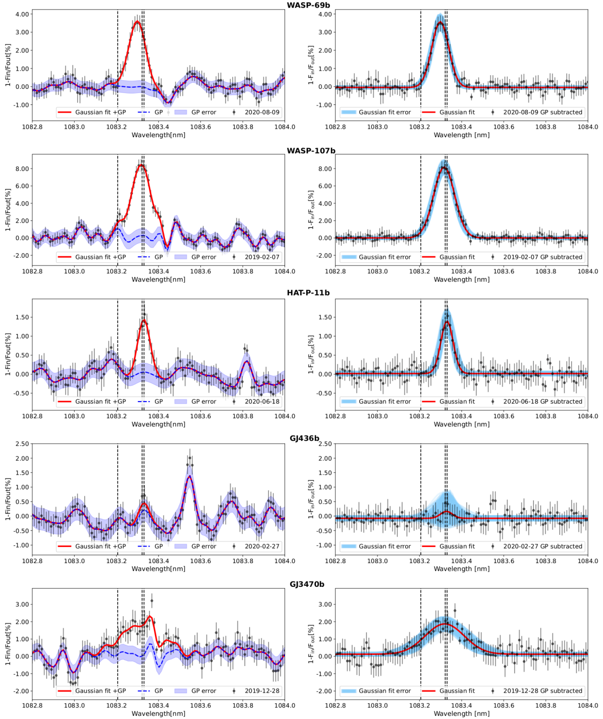
Fig. 4. GP correction. For each target, an example of GP correction is shown. Left panel: transmission spectrum centred on the He I triplet (in the planet rest frame) with overplotted the GP regression model, along with the 1\sigma uncertainty intervals, (in blue) and the Gaussian+GP model (in red). Right panel: final transmission spectrum after removing the GP model. Vertical black dotted lines indicate the position of the He I triplet. The spike in the right wing of the He I triplet in the GJ 3470 b transmission spectrum is a residual due to the OH emission line. The error intervals for the Gaussian fit were computed by displaying 1000 Gaussian fits within the 1\sigma uncertainties of the derived parameters, spanning the 16–84% quantiles.
