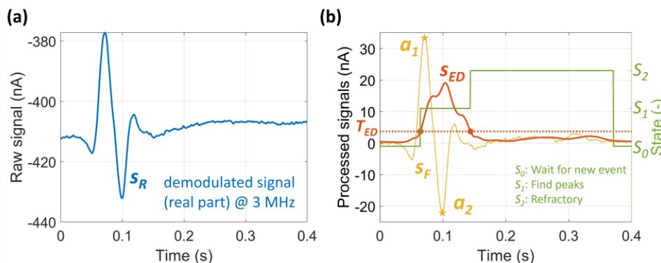
Fig. 2 (a) Exemplary portion of the raw signal ( s_R ) recorded from the MIC sensing zone upon the passage of a particle (i.e., real part of the demodulated differential signal at 3 MHz). The event signal exhibits an asymmetric bipolar shape. (b) Intermediate outcomes of the real-time signal processing algorithm, namely, the high pass filtered signal ( s_F ) and the derived signal ( s_{ED} ) that is used for event detection. The event detection threshold ( T_{ED} ) and the corresponding state are also shown.
