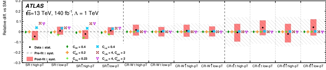
Figure 4. The relative differences between the observed and SM predicted event counts in the SRs and CRs, for both the observed data and the fitted EFT model. The black points represent observed data, with the data statistical uncertainties as uncertainty bars. The grey dashed area indicates the total systematic uncertainties, while the red boxes are centred at positions determined by the best-fit values of the WCs, with heights determined by systematic uncertainties constrained by the fit. The coloured scattered markers correspond to expected values when making various WC assumptions.
