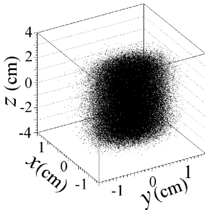
FIG. 4. The reconstructed position of the production vertex.
