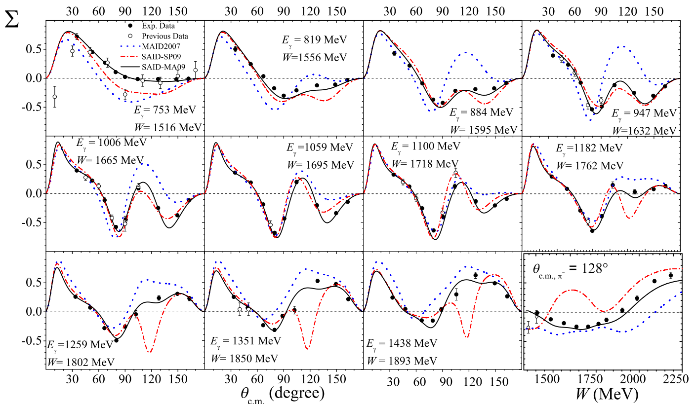
FIG. 8. (Color on line) The beam polarization asymmetries for \gamma n \rightarrow \pi^- p versus pion center-of-mass scattering angle. The photon energy is shown. Solid (dash-dotted) lines correspond to the SAID MA09 (SP09 [26]) solution. Dotted lines give the MAID2007 [27] predictions. Experimental data are from the current (filled circles) and previous measurements [24, 25] (open circles). The plotted points from previously published experimental data are those data points within 4 MeV of the photon energy indicated on each panel. Plotted uncertainties are statistical. In the last panel the asymmetries are plotted versus gamma-ray energy for the CM angle of 128^\circ . The MA09 includes in its database the Graal asymmetries for the \gamma n \rightarrow \pi^- p and \gamma n \rightarrow \pi^0 n [12] reactions. SP09 and MAID2007 do not include these data.
