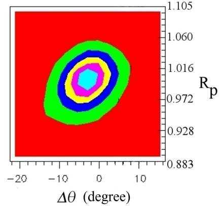
FIG. 3. (Color on line) the bi-dimensional distribution of \Delta\theta vs. R_p as defined in this article.
