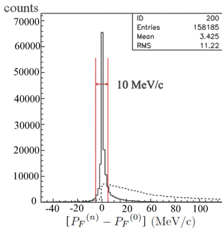
FIG. 2. (Color on line) difference between the Fermi momentum reconstruction at the nth step of recursive method and at step zero for the signal (solid line) and for the concurrent channels (dashed line) in simulation.
