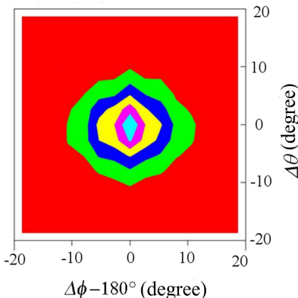
FIG. 5. (Color on line) the bi-dimensional distribution of \Delta\theta vs. \Delta\phi - 180^\circ = |\phi_{\pi^-} - \phi_p| - 180^\circ as defined in this article.
