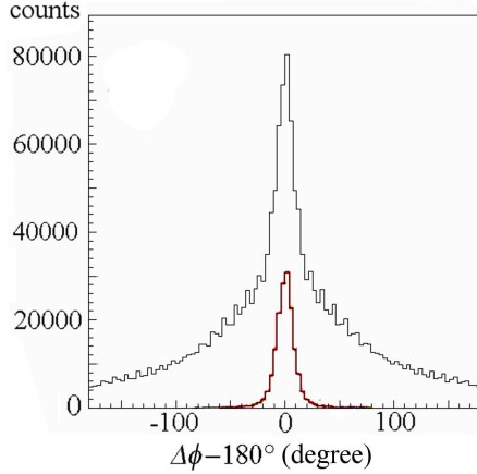
FIG. 1. (Color on line) a) the \pi^- -p coplanarity before (upper curve) and after the cuts (lower curve).
