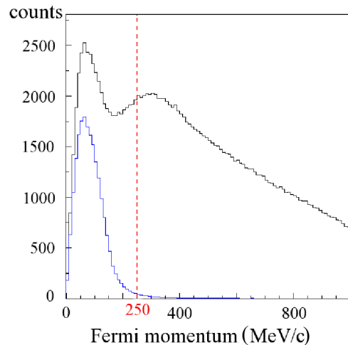
FIG. 6. (Color on line) the Fermi momentum of the neutron calculated before (upper curve) and after (lower curve) the cuts.
