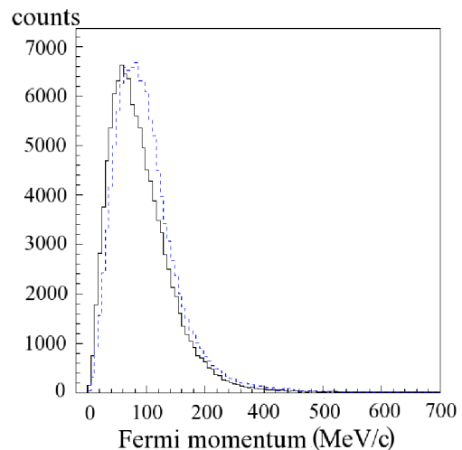
FIG. 7. (Color on line) the Fermi momentum (dashed line) of the neutron after the cuts (data) and that (solid line) generated using the Paris potential.
