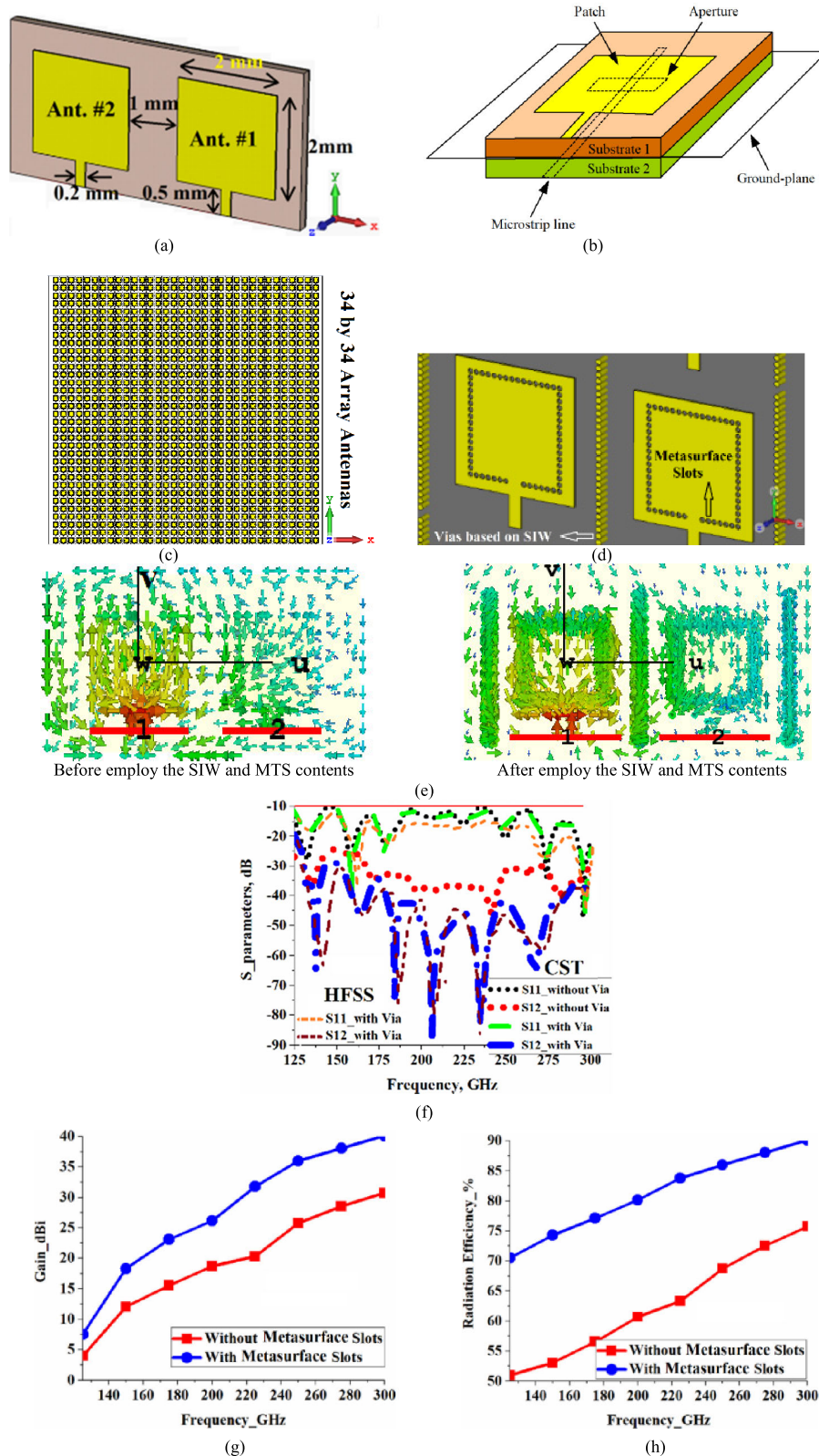
FIGURE 19. (a) Reference 1 × 2 array antenna, (b) feeding structure, (c) layout of whole 34 × 34 array antennas inspired SIW and MTS concepts, (d) zoomed view to depict two central antennas after apply the SIW and MTS principles, (e) surface current density distribution before and after applying the SIW and MTS properties at 250 GHz for two central antennas, (f) S-parameter responses, (g) gain curve, (h) efficiency curve, (i) 3-D radiation diagrams, and (j) co- and cross-polarized radiation gain patterns [131].
