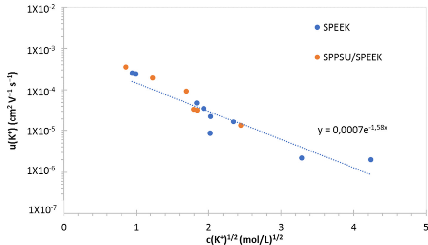
Figure 7. K^+ ion mobility in various proton exchange membranes based on SPEEK and SPPSU/SPEEK blends.
