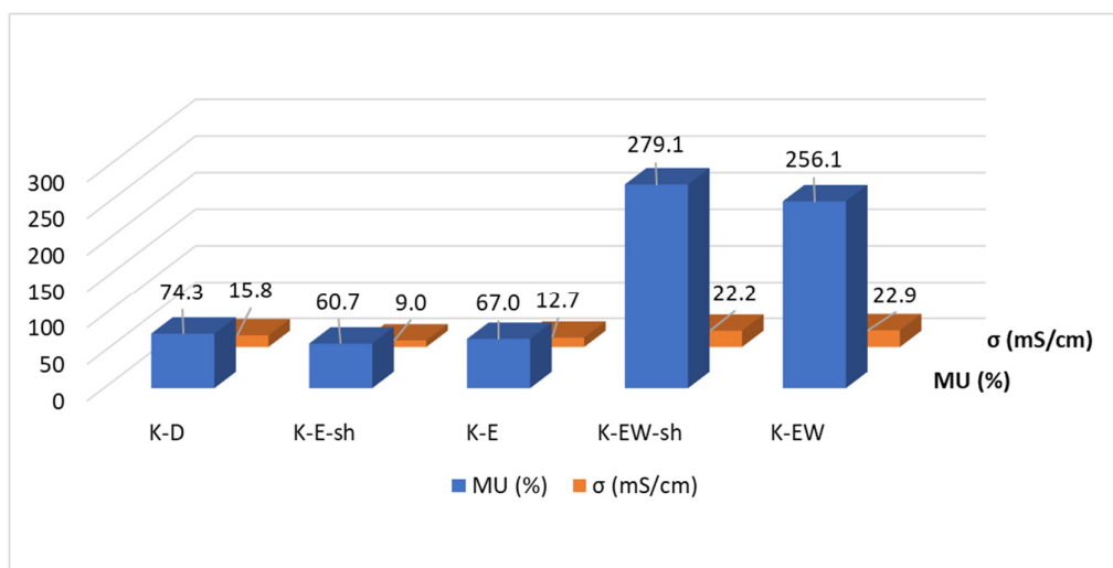
Figure 4. Comparison of SPEEK membranes realized with different solvents and casting procedures.
