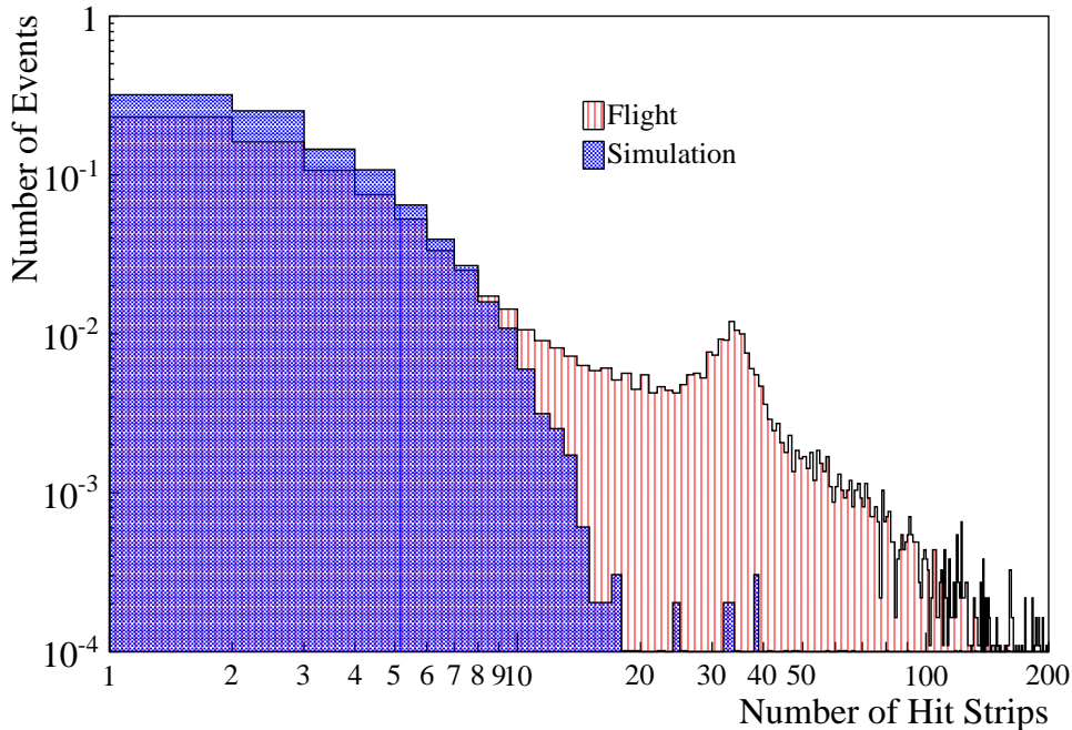
Fig. 4.— The normalized number of hit strips in the last 18 calorimeter planes for events selected with Criteria 1-7 and rigidity between 70 and 150 MV for experimental (red histogram) and simulated (blue histogram) data. The total number of events in both histograms is normalized to 1. The tail to higher values in the number of hit strips for the experimental histogram is associated with a contamination of spillover protons traversing most of the calorimeter, with the peak around 35 due to non-interacting ones.
