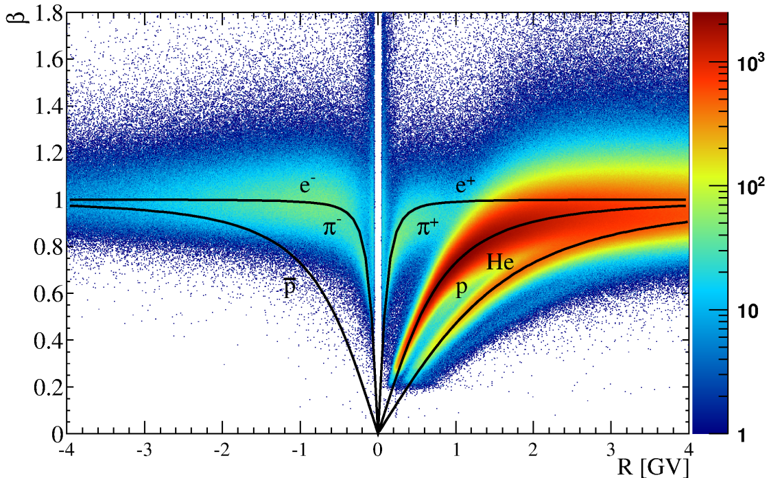
Fig. 2.— ToF velocity ( \beta ) as a function of the rigidity. The various particle species are indicated.
