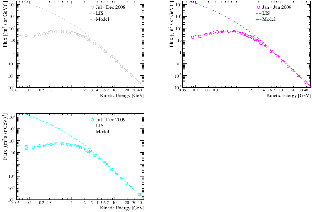
Fig. 17.— The measured electron ( e^- ) energy spectrum for the last three half-year periods from the second half of 2008 to the end of 2009. Time progresses from top to bottom, left to right. The error bars are the quadratic sum of the statistical and systematic errors. If not visible, they lie inside the data points. The computed spectra (solid lines) and the LIS used for the computation (dashed line) are also shown.
