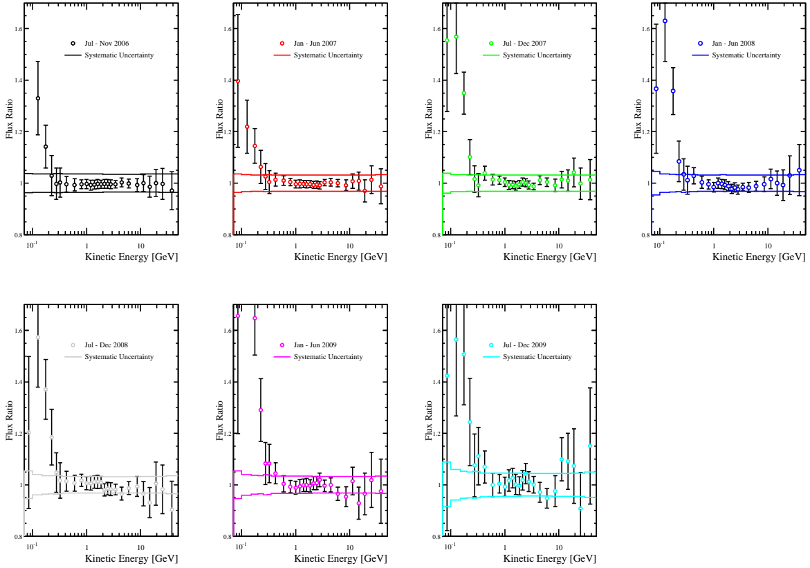
Fig. 13.— The electron fluxes measured in each time interval obtained with Criterion 2 divided by the equivalent ones obtained with Criterion 2bis. The solid lines indicate the systematic uncertainties associated with these data.
