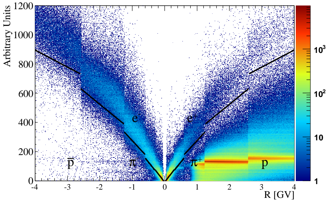
Fig. 3.— A quantity related to the topological development of the shower in the calorimeter as a function of rigidity for events selected with Criteria 1-7. The quantity computation uses the number of the plane closest to the shower maximum estimated for an electromagnetic shower of a given energy. The quantization of the plane numbers produce the shown discontinuities. The events above the solid lines are tagged as electrons by this selection.
