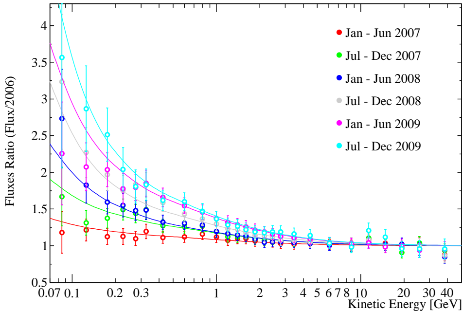
Fig. 18.— The ratios as a function of energy between the measured half-years ( e^- ) fluxes from January 2007 till December 2009 and the measured fluxes for the period July-November 2006 overlaid with the corresponding computed spectra (solid lines). The error bars are the quadratic sum of the statistical and systematic errors.
