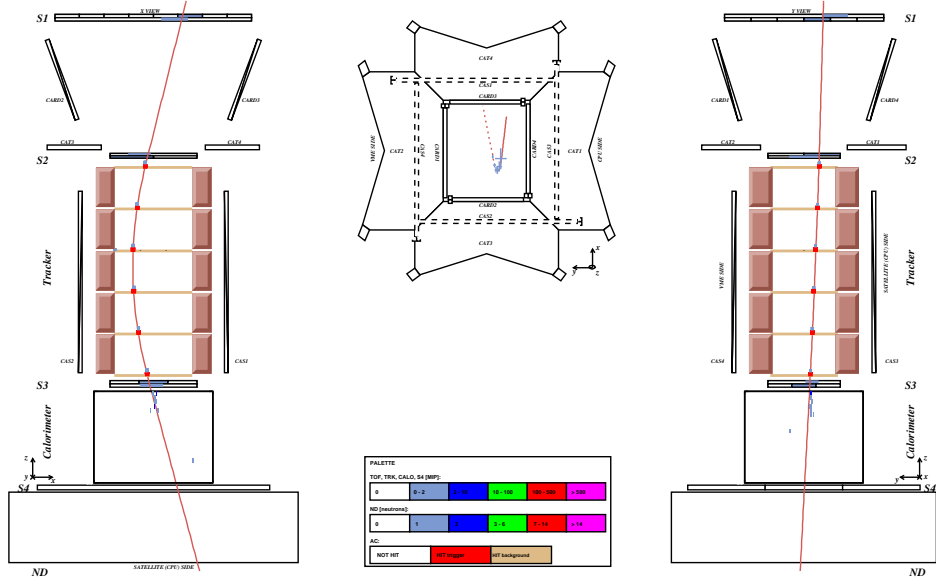
Fig. 5.— The event display of an electron event of \sim 120 MV selected as having a low value in the experimental distribution of Figure 4 . The bending (x) and non-bending (y) views are shown on the left and on the right, respectively. A plan view of PAMELA is shown in the center. The signal as detected by PAMELA detectors are shown along with the particle trajectory (red solid line) reconstructed by the fitting procedure of the tracking system.
