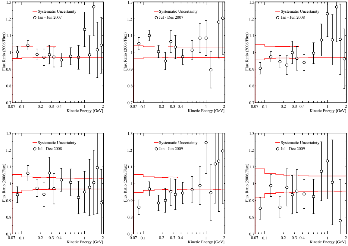
Fig. 14.— The re-entrant albedo e^- fluxes measured in July-November 2006 divided by the equivalent fluxes measured in the other time intervals. The solid lines indicate the systematic uncertainties associated with these data.
