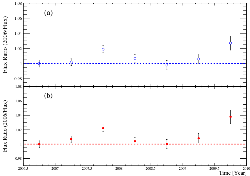
Fig. 12.— The high-energy (30-50 GeV) proton flux measured in July-November 2006 divided by the proton fluxes measured in each time interval. Proton events were selected with the same requirements of the electron analysis but the calorimeter selection using Criterion 2bis (a) and Criterion 2 (b).
