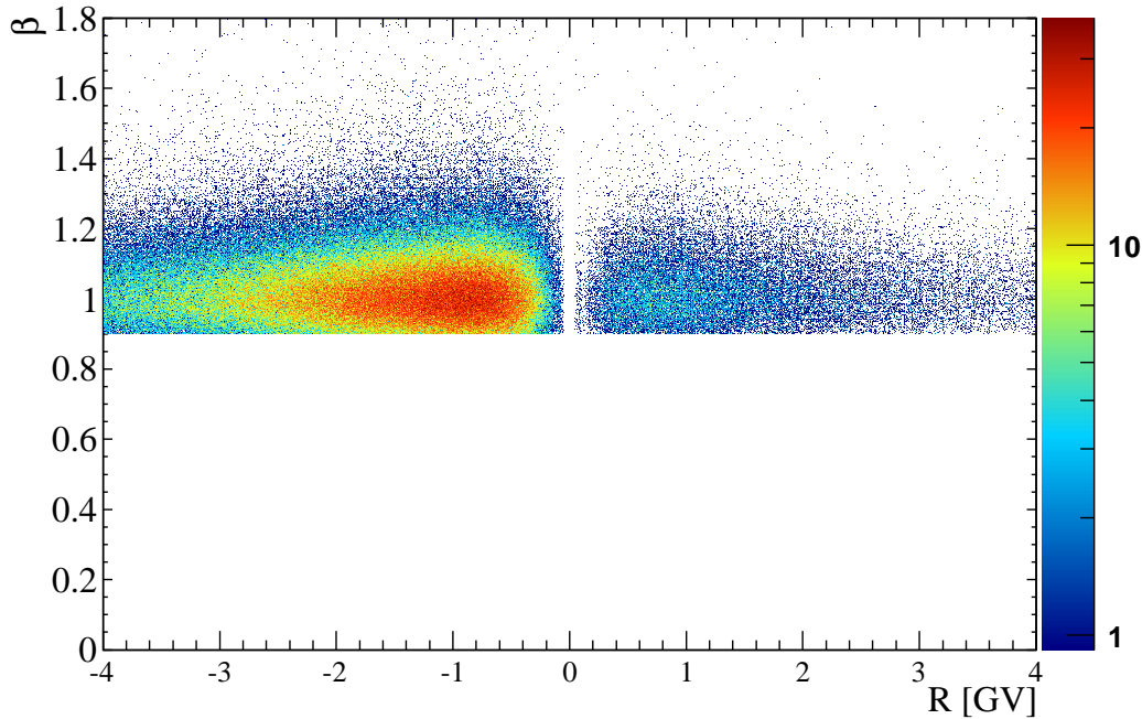
Fig. 7.— ToF Velocity ( \beta ) as a function of the rigidity for the events surviving all selection criteria, included Criterion 7: \beta > 0.9 .
