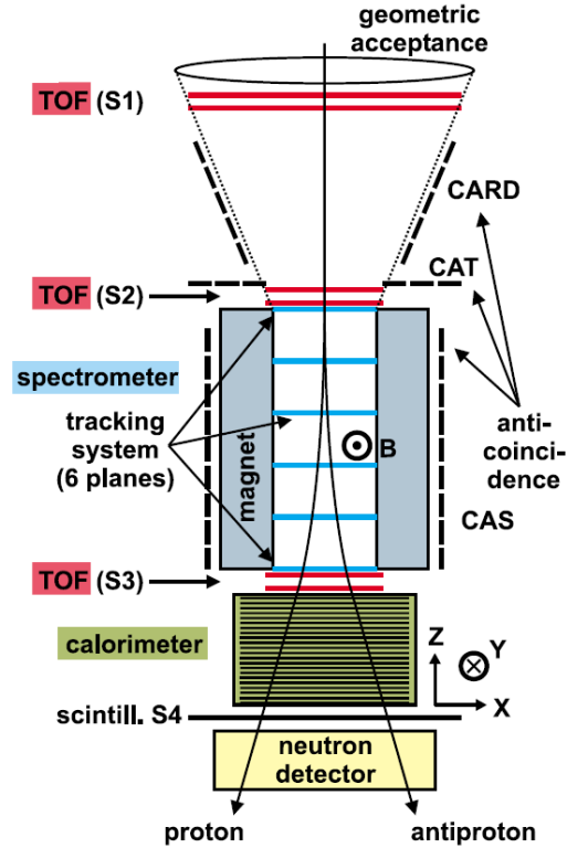
Fig. 1.— Schematic view of the PAMELA apparatus.
