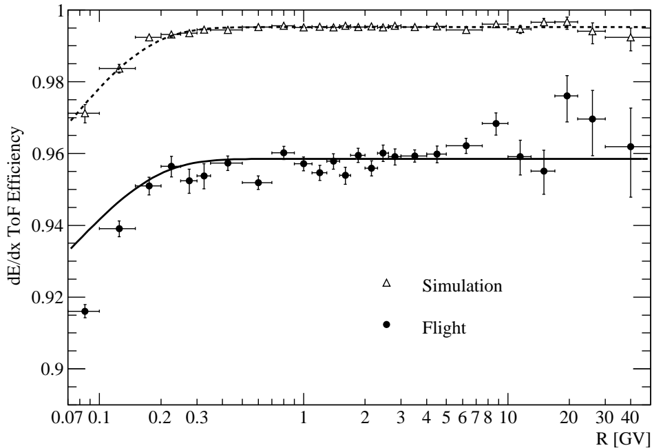
Fig. 8.— Efficiency of the ToF dE/dx selection (Criterion 5) as a function of rigidity for the first time interval (July–November 2006) for flight (full circles) and simulated (open triangles) data. The dashed line is a fit to the simulated data; the solid line is a fit to the experimental data based on the simulated shape and indicates the efficiency used in the data analysis.
