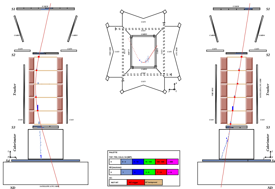
Fig. 6.— The event display of a spillover proton event of \sim 110 MV selected from the peak around 35 in the experimental distribution of Figure 4 . See Figure 5 for further details.
