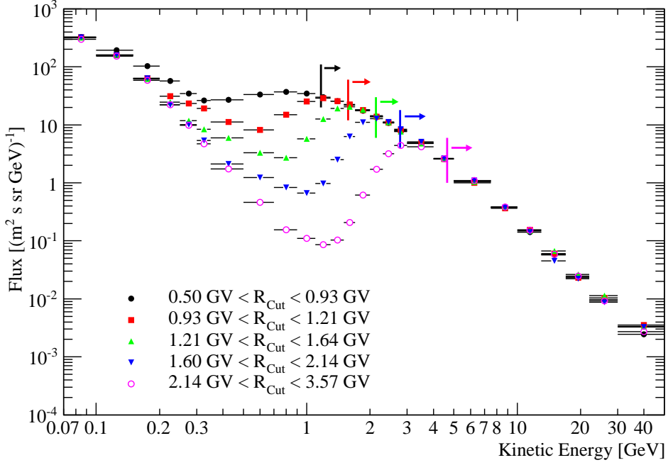
Fig. 11.— Electron ( e^- ) energy spectrum measured by PAMELA at the five geomagnetic rigidity cutoff ( R_{\text{Cut}} ) intervals specified in the figure. The arrows indicate the energy regions where the galactic electrons dominate and are unaffected by the Earth’s magnetosphere. Around the geomagnetic cutoff, in the penumbral region, galactic electrons are mixed with re-entrant albedo electrons that become the dominant component as the energies decrease. satellite at high geomagnetic latitudes.
