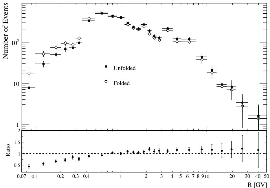
Fig. 10.— Top panel: distributions of the event counts, corrected for all selection efficiencies except those of selection Criteria 2 and 4, selected in the lowest geomagnetic cutoff interval ( 0 - 0.055 GV) before (open circles) and after (full circles) the unfolding procedure. Bottom panel: ratio between the unfolded and folded count distributions.
