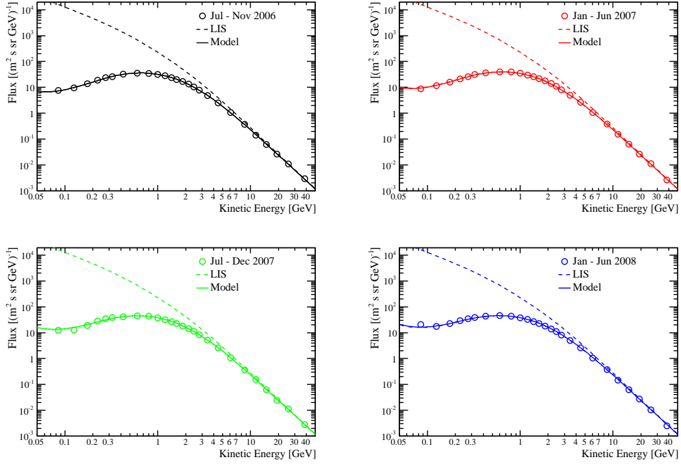
Fig. 16.— The measured electron ( e^- ) energy spectrum for the first half-year periods from the second half of 2006 to the first half of 2008. Time progresses from top to bottom, left to right. The error bars are the quadratic sum of the statistical and systematic errors. If not visible, they lie inside the data points. The computed spectra (solid lines) and the LIS used for the computation (dashed line) are also shown.
