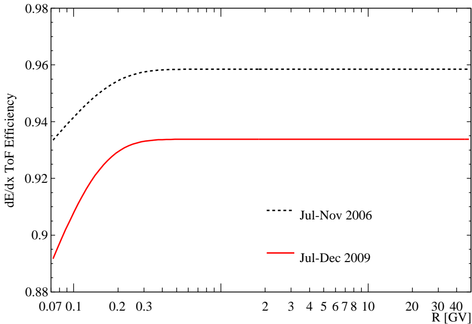
Fig. 9.— Temporal evolution of the ToF dE/dx selection efficiency. Black dashed line: efficiency for the first time interval (July-November 2006), red solid line: efficiency for the last time interval (July-December 2009).
