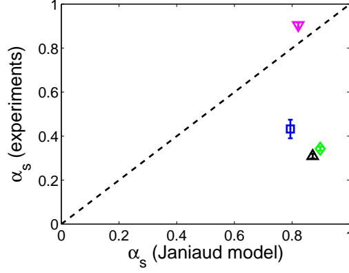
FIGURE 6. Relative slip measured in the experiments described in Tab. 1, as a function of the relative slip (4.8) predicted by the model of Janiaud, Weaire & Hutzler (2006).
