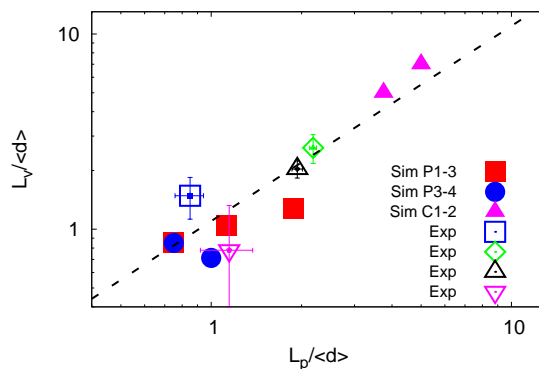
FIGURE 11. Scatter plot of the shear localisation length L_v (computed from a hyperbolic cosine fit of the velocity profiles) vs the plastic localisation length L_p (computed out of an exponential fit of the symmetrised rate of plastic events across the channel) for three sets of data: experiments (symbols as in Tab. 1), simulations of Poiseuille flow with fixed pressure drop and various \beta^* 's (filled squares) and with fixed \beta^* = 200 and various pressure drops (filled circles) and simulations of Couette flow at two \beta^* 's (filled triangles); both lengths are normalised by the mean bubble diameter. The dashed line is the L_v = L_p curve.
