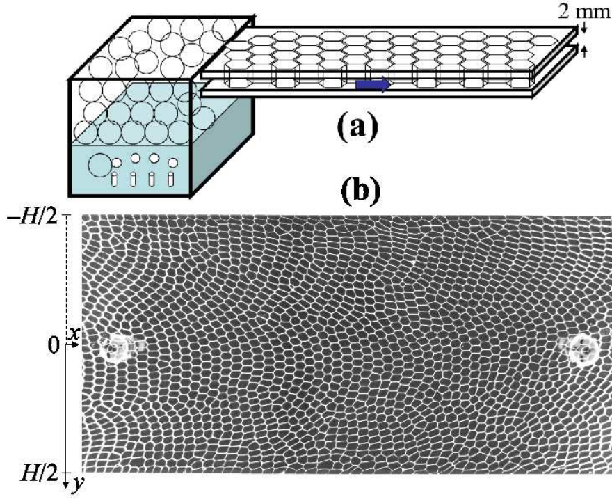
FIGURE 1. (a) Sketch of the side view of the setup. (b) Snapshot of an experiment. The distance between the two side walls is H = 106.6 mm. The average bubble size is 12.3 \text{ mm}^2 and the liquid fraction is \phi_l = 4.8\% . The two spots at the left and right of the image are the points between which the pressure drop is measured.
