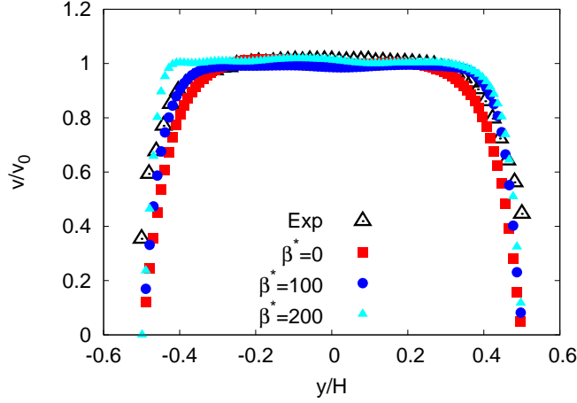
FIGURE 8. Numerical velocity profiles, normalised by the centreline velocity v_0 , at changing the friction constant. Data from three sets of simulations are shown with dimensionless friction parameter (see equation 4.15) \beta^* = 0, 100, 200 (runs P1-3 in table Tab. 2); the experimental velocity profile with flow rate 152.5 ml/min (see Tab. 1) is also reported to show that we are able to tune the friction parameters in the numerics to achieve the same localisation observed in the experiments. The equivalent \beta^* in the experiments is \beta^* \approx 250 (see text for details). On the abscissae, the y -location across the channel has been normalised by the total channel height.
