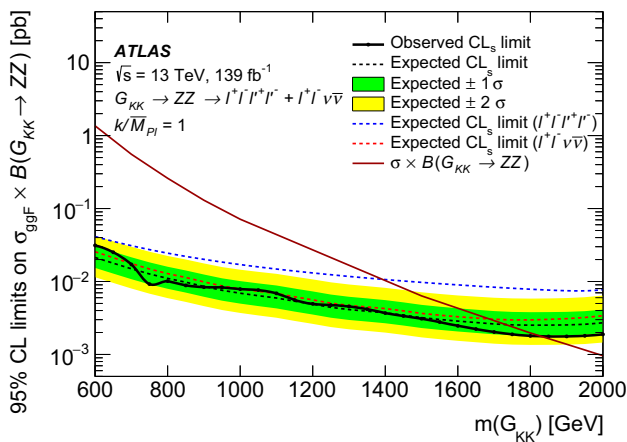
Fig. 8 The upper limits at 95% CL on cross section times branching ratio \sigma \times B(G_{\text{KK}} \rightarrow ZZ) for a KK graviton produced with k/\bar{M}_{\text{Pl}} = 1 . The black line indicates the observed limit. The green and yellow bands give the \pm 1\sigma and \pm 2\sigma uncertainties in the expected limits. The predicted production cross section times branching ratio as a function of the G_{\text{KK}} mass m(G_{\text{KK}}) is shown by the red solid line
