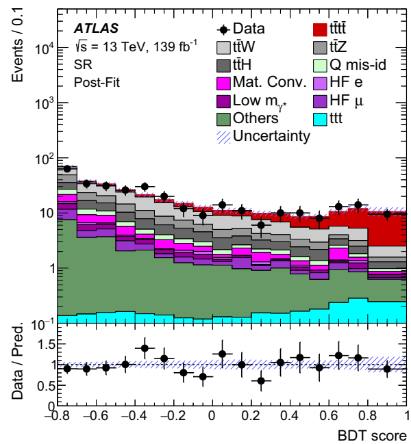
Fig. 3 Comparison between data and prediction after the fit (‘Post-Fit’) for the distribution of the BDT score in the SR. The band includes the total uncertainty of the post-fit computation. The ratio of the data to the total post-fit computation is shown in the lower panel. See Sect. 5 for the definitions of the different background categories
