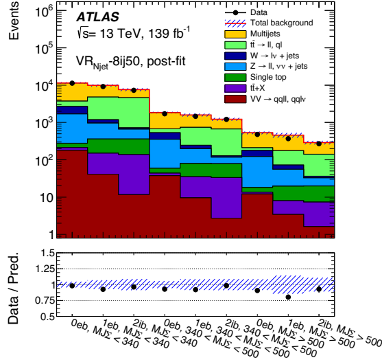
(a) VR_{N_{jet}}
