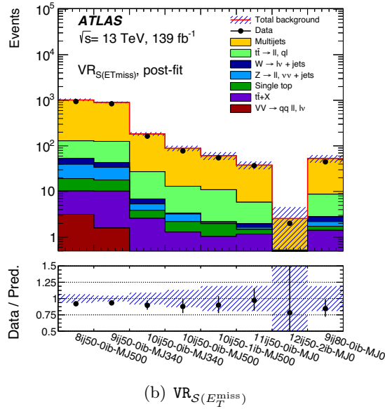
Figure 7. Post-fit event yields in validation regions summarised for all single-bin signal regions. The upper panel shows the absolute yields for data (black points) and all background subcomponents (histograms), with the combination of statistical and systematic uncertainties shown by the hatched areas. The lower panel shows the ratio of the data yields to the total SM prediction.
