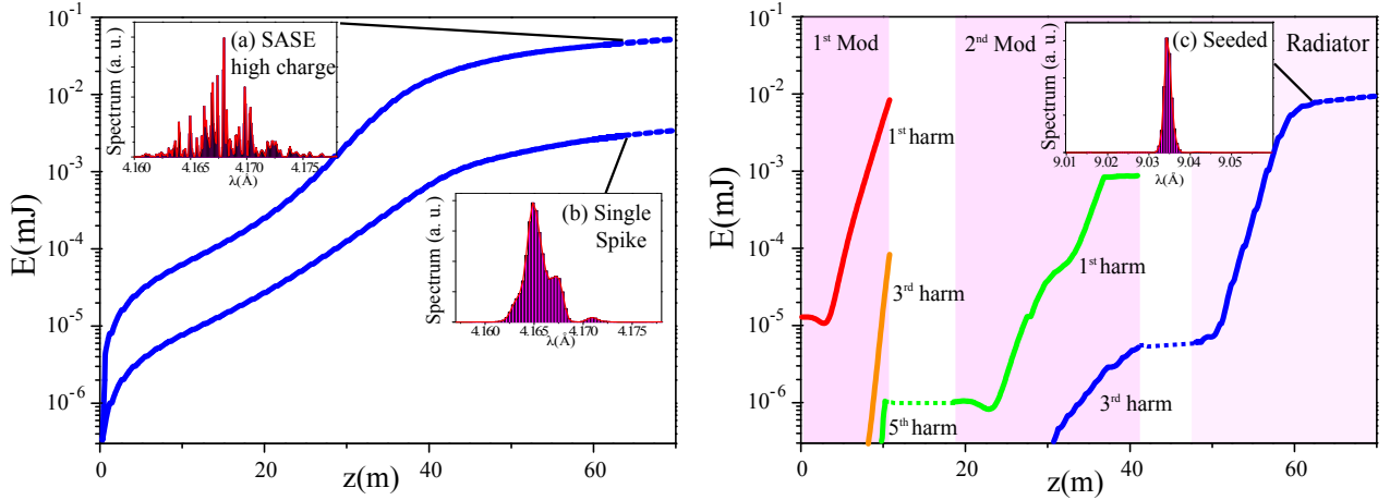
Figure 4: FEL radiation energy vs undulator position and spectra (in the boxes) extracted at 60 m. Left window: (a) SASE case obtained in UliX2 with Q=50 pC. (b) SASE single spike, same parameters as (a), but Q=8 pC. Right window: (c) Seeded cascaded fresh-bunch case. First modulator (1 st Mod) with 5 cm period. Second modulator (2 nd Mod) with 2.8 cm period. Radiator with 1.2 cm period. The FEL simulations have been performed with GENESIS 1.3 [18].
