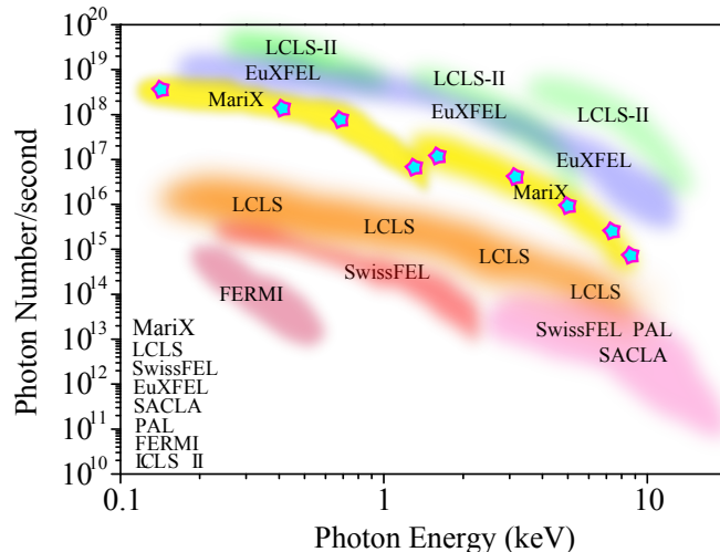
Figure 5: The expected performances of MariX Free Electron Laser (yellow area), in terms of photon flux as a function of the photon energy in the 0.2-8 keV anticipated dynamic range, showing performances above present FELs driven by normal conducting Linacs, second only to the anticipated performances of LCLS-II and EuXFEL.
