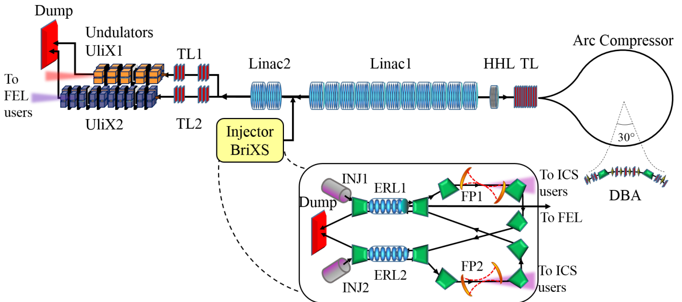
Figure 1: Conceptual lay-out for MariX, based on a two-pass CW Super-Conducting CW GeV-class Linac driven by a folded push-pull Energy Recovery 100 MeV Linac.
