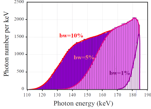
Figure 3: Inverse Compton Scattering spectra. Photon yield as function of the photon energy. Collimation angles respectively 0.6, 2.1, 3.3 mrad for increasing bandwidths.
