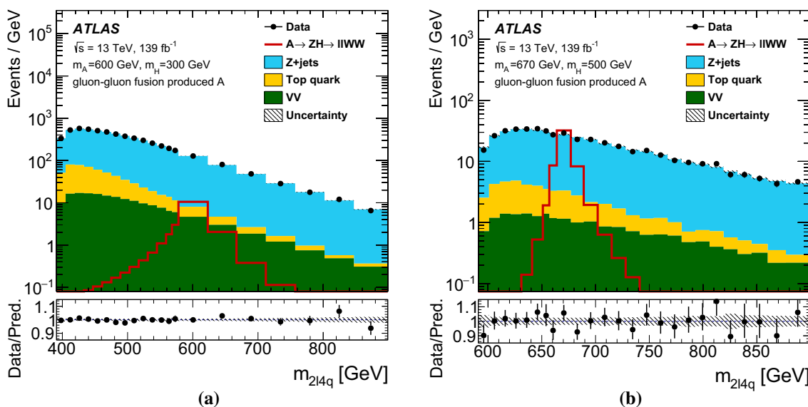
Fig. 12 The m_{2l4q} mass distribution for the m_{4q} windows defined for a m_H = 300 GeV and b m_H = 500 GeV. Signal distributions are also shown with (m_A, m_H) = (600, 300) GeV and (m_A, m_H) =
