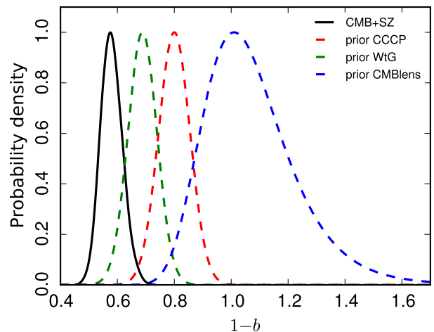
Fig. 8: Comparison of cluster and primary CMB constraints in the base \Lambda CDM model, expressed in terms of the mass bias, 1-b . The solid black curve shows the distribution of values required to reconcile the counts and primary CMB in \Lambda CDM; it is found as the posterior on 1-b from a joint analysis of the Planck cluster counts and primary CMB when leaving the mass bias free. The coloured dashed curves show the three prior distributions on the mass bias listed in Table 2.
