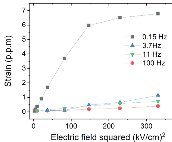
Fig. 2 Electromechanical strain of the CGO single crystal at room temperature for different electric field frequencies measured by laser interferometry (Fig. S1, ESI†). The electrostriction coefficients are reported in Table 1.
