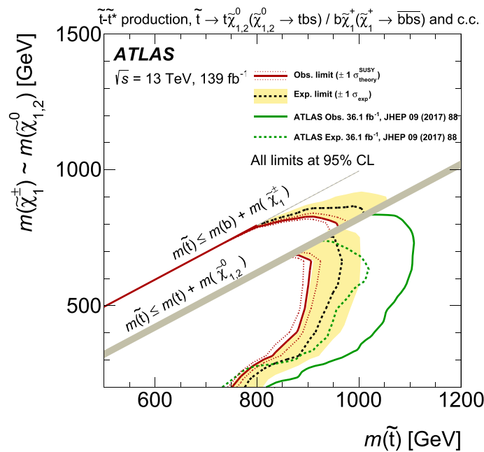
Fig. 8 Observed and expected exclusion contours for the \tilde{t} and \tilde{\chi}_1^{\pm} masses in a top-squark production model with RPV decays of the \tilde{\chi}_1^{\pm} and of the \tilde{\chi}_{1,2}^0 . Limits are shown in the case of a higgsino LSP. The contours of the band around the expected limit are the \pm 1\sigma variations, including all uncertainties except theoretical uncertainties in the signal cross-section. The dotted lines around the observed limit illustrate
