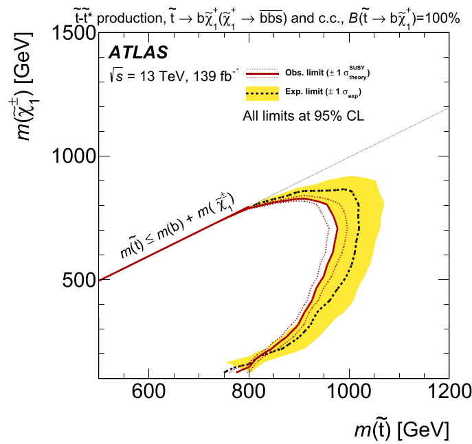
Fig. 7 Observed and expected exclusion contours for the \tilde{t} and \tilde{\chi}_1^{\pm} masses in a top-squark production model with RPV decays of the \tilde{\chi}_1^{\pm} . Limits are shown for B(\tilde{t} \rightarrow b\tilde{\chi}_1^+) equal to unity. The contours of the band around the expected limit are the \pm 1\sigma variations, including all uncertainties except theoretical uncertainties in the signal cross-section.
