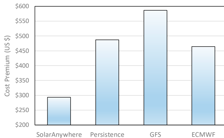
Figure 5. Comparing firm forecast cost premium per nominal KW as a function of the forecast model. Displayed costs represent a mean for all scenarios and time horizons analyzed.
