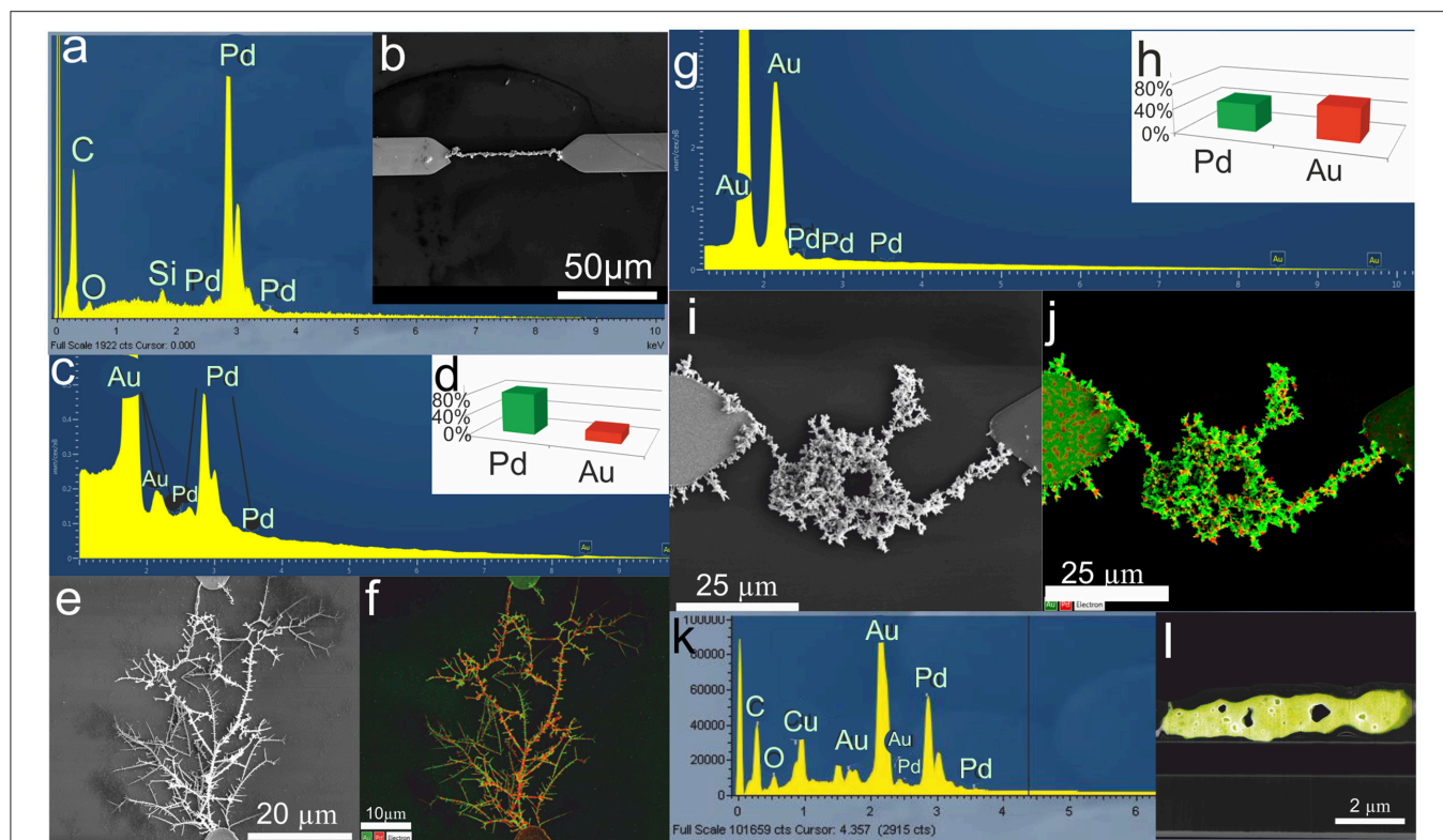
FIGURE 3 | (a) EDX spectrum of a Pd NW electrode. (b) SEM micrograph of the Pd NW electrode shown in (a). The Pd NW electrode was synthesized by electrodeposition from a Pd ( \text{ac}_2 ) solution. (c) EDX spectrum of a Pd-Au nanodendrite electrode and (d) histogram of the Pd and Au element content in the Pd-Au nanodendrite shown in (e) the SEM micrograph. (f) SEM micrograph of the same Pd-Au nanodendrite electrode with elemental mapping (Pd-green, Au-red). The Pd-Au nanodendrite electrode was electrochemically assembled in a 5 \times 10^{-3} M \text{HAuCl}_4 and 5 \times 10^{-3} M \text{K}_2\text{PdCl}_4 water solution at 45 MHz, 17 V_{pp} , and 1.5 V DC offset. (g) EDX spectrum of a Pd-Au nanodendrite electrode and (h) histogram of the Pd and Au element content in the Pd-Au nanodendrite electrode shown in (i) the SEM micrograph. (j) EDX elemental mapping of the same Pd-Au nanodendrite electrode (Pd-green, Au-red). (k) EDX spectrum of the lamella (cross section) of the Pd-Au nanodendrite electrode. (l) EDX elemental mapping of the same lamella of the Pd-Au nanodendrite electrode. The structure was synthesized by electrodeposition from 5 \times 10^{-3} M \text{HAuCl}_4 and 5 \times 10^{-3} M \text{PdCl}_2 dissolved in PBS, pH 8, at 38 MHz, 17 V_{pp} , and 1.5 V DC offset. Reprinted by permission from: Springer, J. Solid State Electrochemistry, Bimetallic nanowire sensors for extracellular electrochemical hydrogen peroxide detection in HL-1 cell culture, Konstantin G. Nikolaev, Vanessa Maybeck, Elmar Neumann, Sergey S. Ermakov, Yury E. Ermolenko, Andreas Offenhäusser, Yulia G. Mourzina © (2017), advance online publication, 28.11.2017 (doi: 10.1007/s10008-017-3829-3).
