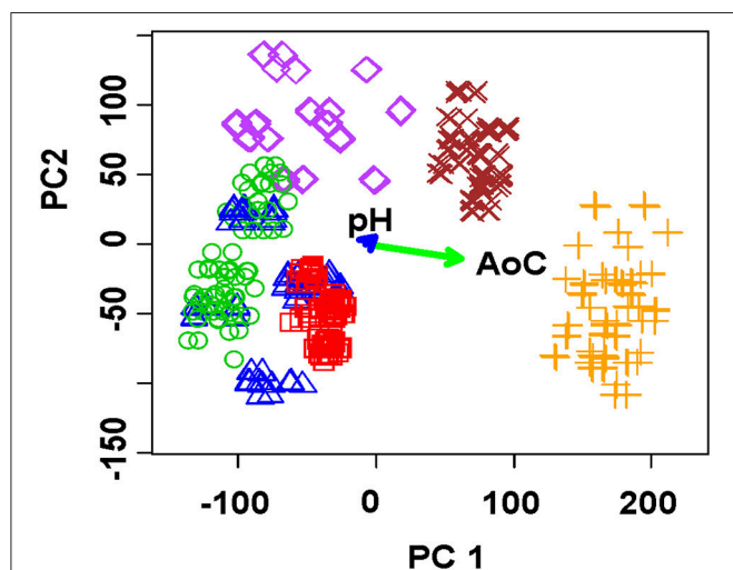
FIGURE 6 | PCA scores plot (two first principal components) of apple juice brands obtained with the ET system comprising of nine solid-contact ISEs on the base of the polyaniline and thiacalix[4]arene ionophores. AoC—antioxidant capacity. Two sample dilutions (1:70 and 1:100) and one Fe(III) concentration (1.0 mM) (Evtugyn et al., 2010), with permission of Elsevier.
