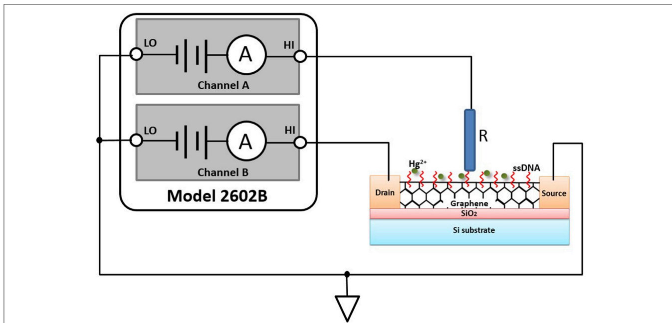
FIGURE 1 | GFET sensor test configuration using multiple SMUs, Model 2602B: HI is short for Force HI terminal, and LO is short for Force LO terminal. R in the figure is an external Ag/AgCl reference electrode with saturated KCl.
