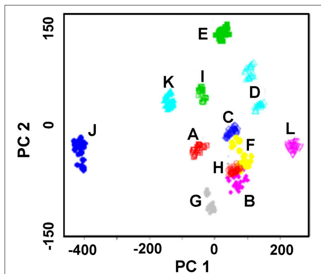
FIGURE 7 | PCA scores plot (two first principal components) of green tea infusions obtained with the ET system comprising of nine solid-contact ISEs on the base of the polyaniline and thiacalix[4]arene ionophores. Sample dilutions 1:1 and 1:20, Fe(III) concentration 0.1 and 1.0 mM. Reproduced from Evtugyn et al. (2011a) with permission of J.Wiley & Sons.
