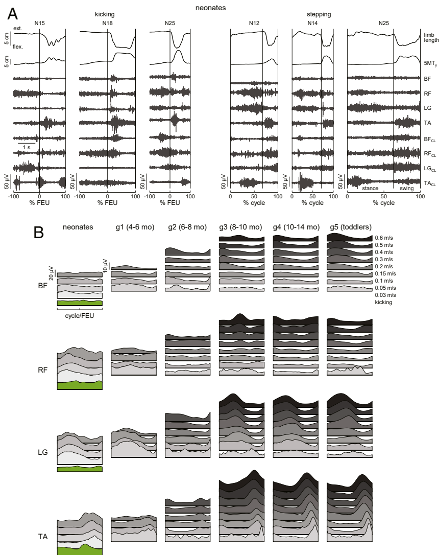
Fig. 1. Recorded EMG profiles during stepping and kicking. (A) Examples of foot motion and raw EMGs in different neonates. Limb length, distance between GT and LM markers; SMT y , y coordinate of 5MT-marker; CL, contralateral leg muscles. Stepping includes stance and swing (vertical line marks transition). Kicking includes a flexion–extension unit (FEU) and a time-epoch just preceding and of the same duration as the FEU. Time scale for all panels in the leftmost panel. (B) Ensemble-averaged (across all cycles of all subjects of each group) rectified, filtered EMG profiles aligned with stance onset (stepping), or –100% FEU (kicking) are plotted over a normalized time base. Bottom to Top : Kicking in neonates (green), stepping at increasing treadmill speeds (grayscale). Data refer to pooled cycles from all neonates kicking supine and all children stepping on treadmill. g1, 4- to 6-mo infants; g2, 6 to 8 mo; g3, 8 to 10 mo; g4, 10 to 14 mo; g5, toddlers, 12 to 15 mo (numbers of subjects in SI Appendix, Supplementary Methods ).
