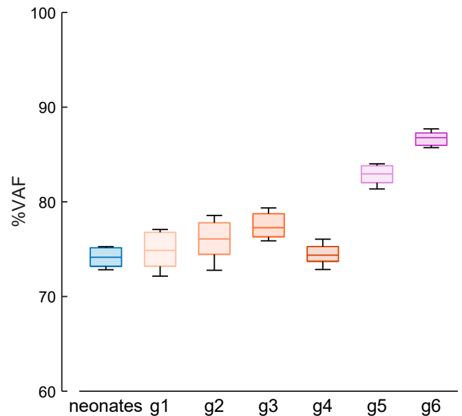
Fig. 6. Reconstruction of EMG activities of stepping children using neonate kicking patterns. Box-and-whisker plots of median and 5th to 95th percentiles (over 100 bootstrap iterations) of the VAF of the reconstruction of the EMGs of each group of children (neonates, g1 to g6); the whiskers extend to the lowest and highest values.
