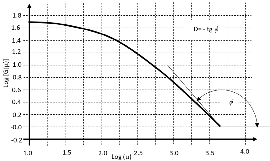
Fig. 2. Richardson's diagram
