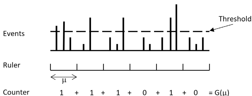
Fig. 1. Box-counting method.
