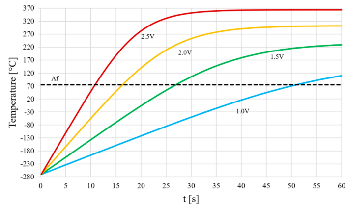
Figure 5. Temperature-Time graph for SMA element in the space environment with different applied voltages.
