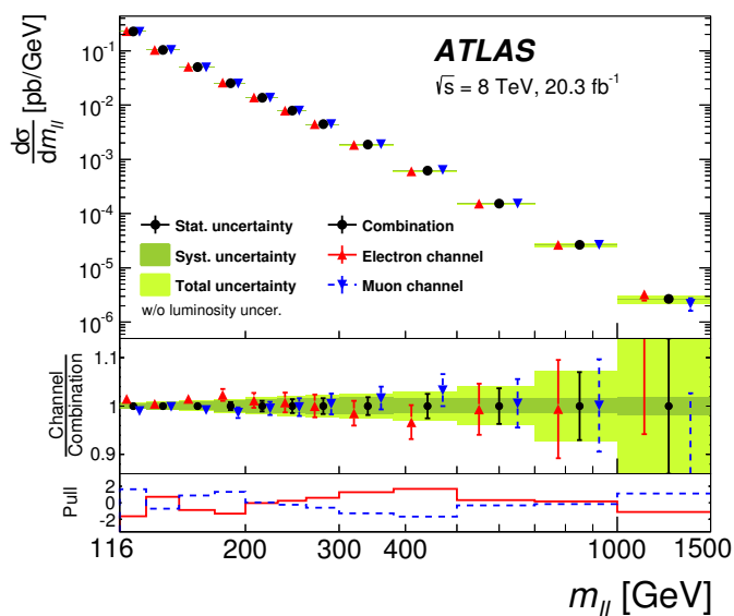
Figure 6. Comparison of the electron (red points), muon (blue points) and combined (black points) single-differential fiducial Born-level cross sections as a function of invariant mass m_{\ell\ell} . The error bars represent the statistical uncertainty. The inner shaded band represents the systematic uncertainty on the combined cross sections, and the outer shaded band represents the total measurement uncertainty (excluding the luminosity uncertainty). The central panel shows the ratio of each measurement channel to the combined data, and the lower panel shows the pull of the electron (red) and muon (blue) channel measurements with respect to the combined data.
