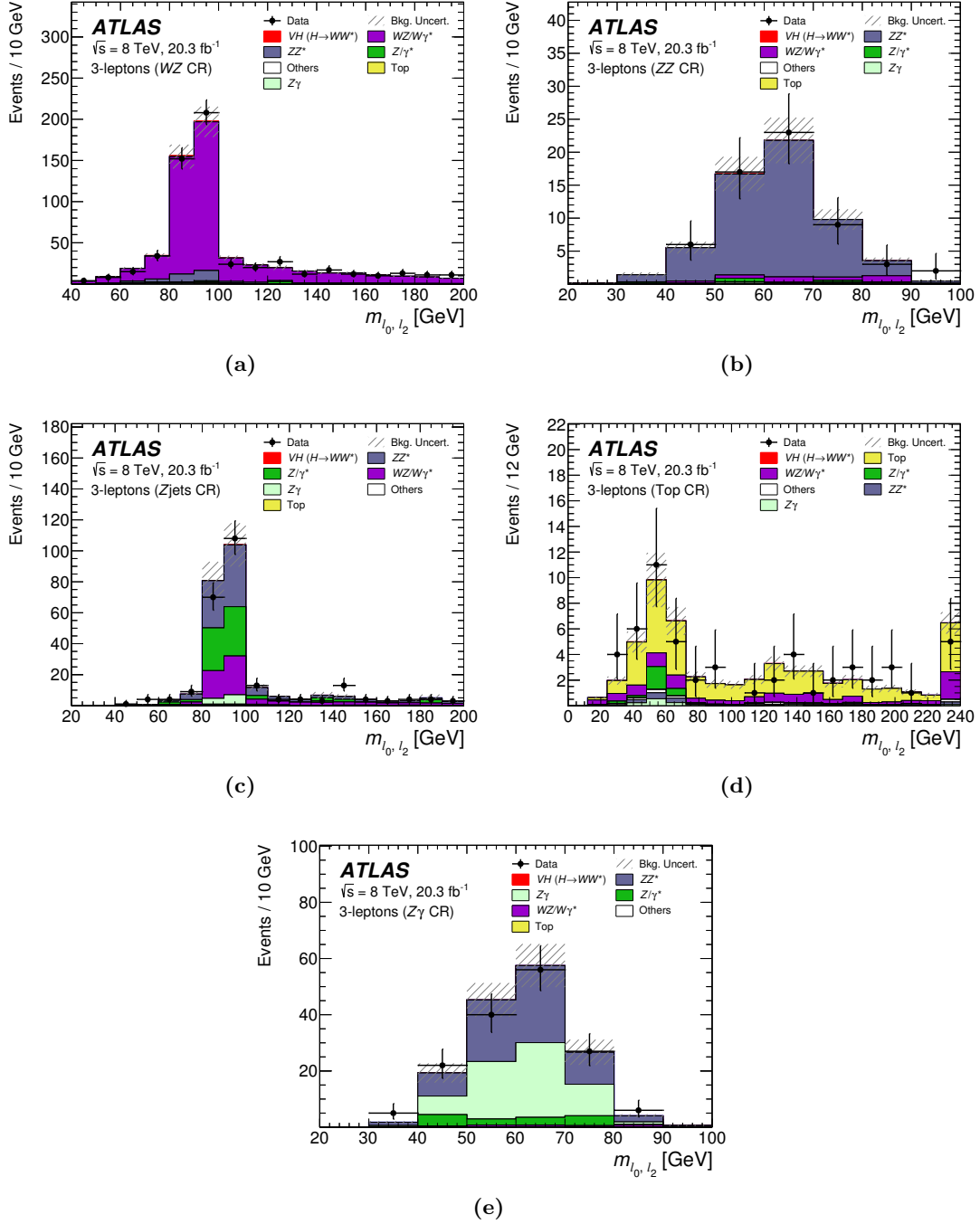
Figure 2. Distributions of the invariant mass of leptons \ell_0 and \ell_2 , defined in section 2, in the five CRs defined in the 3\ell channel: (a) 3\ell -WZ CR, (b) 3\ell -ZZ CR, (c) 3\ell -Zjets CR, (d) 3\ell -Top CR and (e) 3\ell - Z\gamma CR. Data (points) are compared to the background plus VH(H \rightarrow WW^*) ( m_H=125 \text{ GeV} ) signal expectation (stacked filled histograms), where the background contributions are normalised by applying the normalisation factors shown in table 7. The hatched area on the histogram represents total uncertainty, both statistical and systematic (see section 7), on the total background estimate. The last bin includes overflows.
