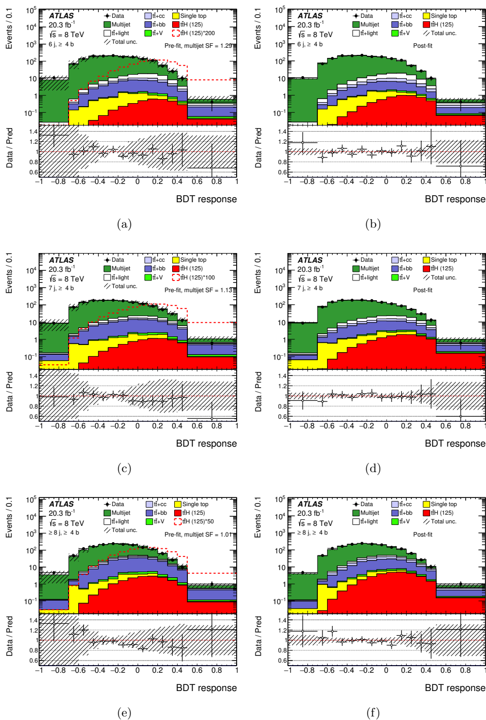
Figure 8. Comparison between data and prediction for the BDT discriminant in the, from top to bottom, (6-8j, \geq 4b ) regions before (left) and after (right) the fit. The fit is performed under the signal-plus-background hypothesis. Pre-fit plots show an overlay of the multijet distribution normalised to data for illustration purposes only. The bottom panels display the ratios of data to the total prediction. The hashed areas represent the total uncertainty in the background predictions. The t\bar{t}H signal yield (solid red) is scaled by a fixed factor before the fit.
