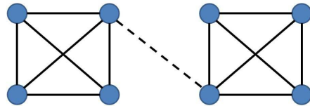
FIG. 1. A simple example to illustrate how an improper spurious link removal method can disconnect a network.
