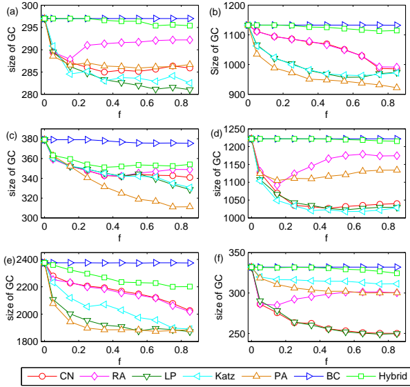
FIG. 3. (Color online) GC’s size when various indices are used to build A^r (here f' = f ) and for different f . The true networks are (a)CE, (b)Email, (c)SC, (d)PB, (e)PPI, (f)USAir. Results are averaged over 100 independent realizations.
