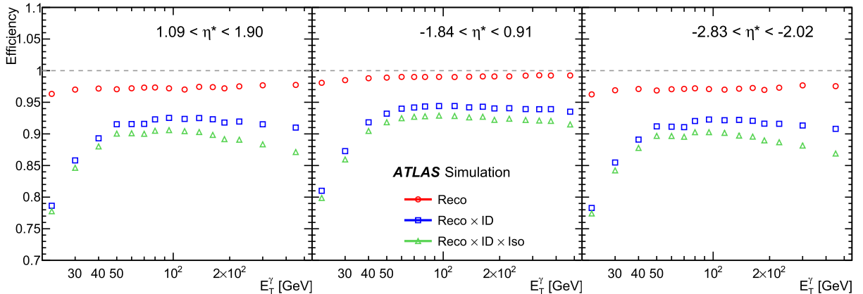
Fig. 2. Efficiency for simulated photons passing the generator-level isolation requirement, shown as a function of photon transverse energy E_T^\gamma with a different pseudorapidity region in each panel. The reconstruction (red circles), reconstruction plus identification (blue squares) and total selection (green triangles) efficiencies are shown separately.
