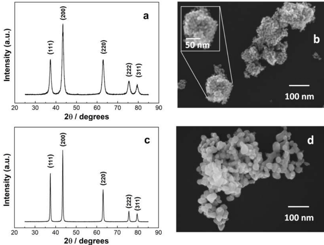
Figure 2. (a) XRD and (b) SEM image of grained-flowers NiO (c) XRD and (d) SEM images of the nanoparticles NiO. The inset in panel (b) is the enlargement of one of the grained-flowers.
