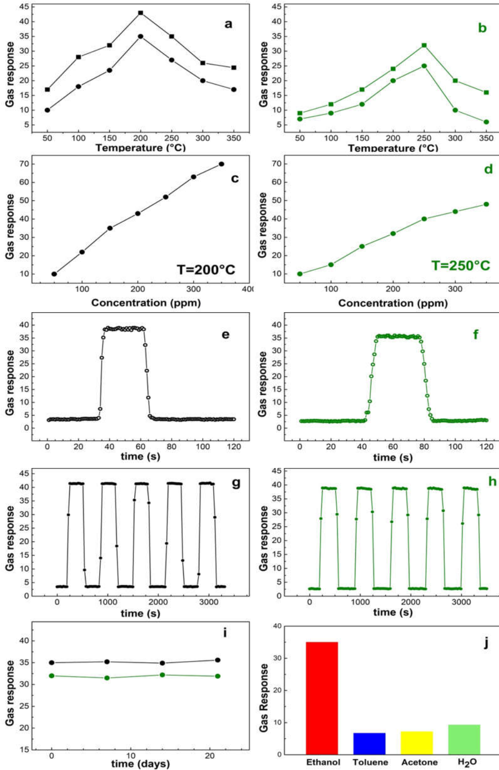
Figure 3. Plots of the gas responses. (a–h): the left panels correspond to grained-flower NiO, the right ones to the NiO nanoparticles. (a, b) are the gas response vs. temperature of sensors exposed to 150-ppm (solid dots) and 200-ppm (solid squares) ethanol, respectively. The gas responses vs. concentration are reported at 200 °C for the grained-flower (c) and 250 °C for the nanoparticles (d). (e, f) are response/recovery time; (g, h) repetitively over time. Panel (i) is the response of the
