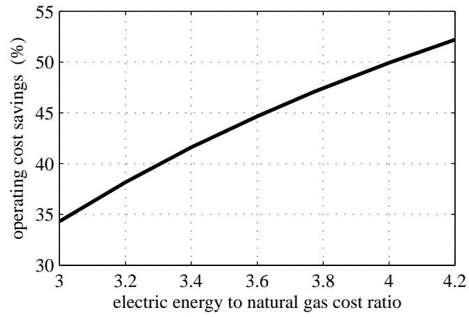
Figure 6: Influence of electric energy to natural gas cost ratio on operating cost savings
