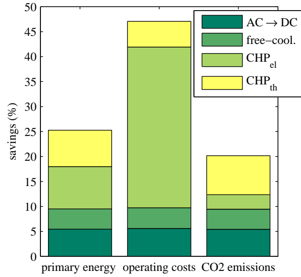
Figure 5: Primary energy, operating costs and CO 2 emission savings for the reference data center located in Rome
