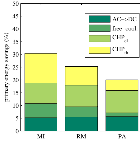
Figure 7: Primary energy savings for the reference data center located in Milan, Rome or Palermo
