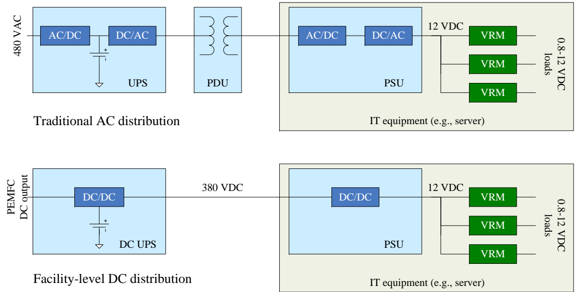
Figure 2: Data center power distribution systems: traditional AC (top) and high-voltage DC (bottom)
