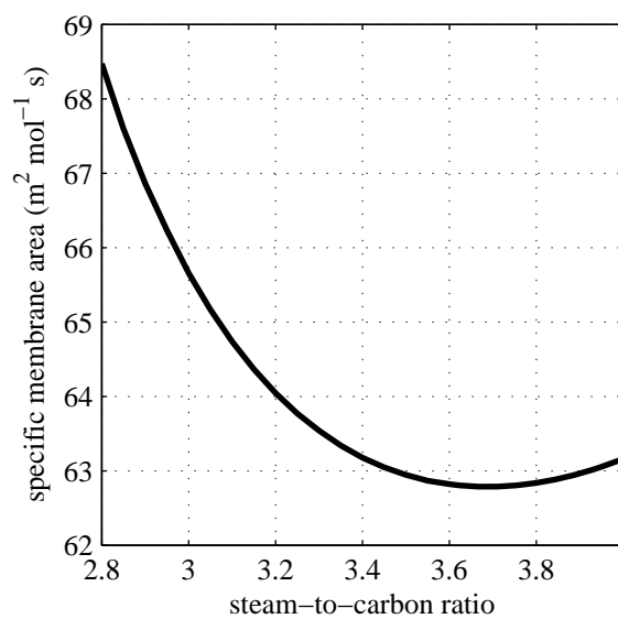
Figure 4: Influence of steam-to-carbon ratio on specific membrane area (with reference to 1 \text{ mol s}^{-1} of natural gas input)
