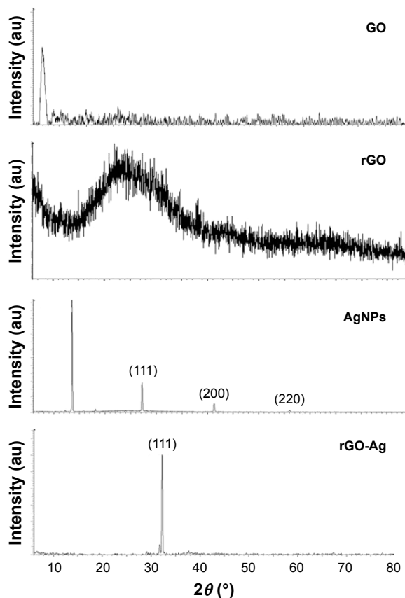
Figure 2 XRD patterns of GO, rGO, and rGO-Ag nanocomposites.
