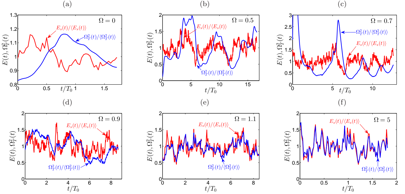
FIG. 6: Color online. The energy (red lines) and enstrophy (blue lines) time evolutions in the subcritical regime normalized by mean-in-time values [Panels (a),(b),(c)] with \Omega = 0, 0.5, 0.7 , the critical [Panel (d), \Omega = 0.9 ] and the supercritical regime [Panels (e),(f)] with \Omega = 1.1, 5.0 ].
