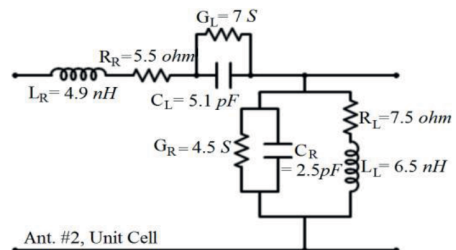
Equivalent circuit of the unit cell in Ant.#2
