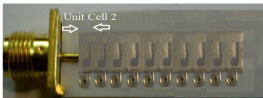
Manufactured prototype of Ant.#2
