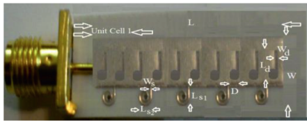
Manufactured prototype of Ant.#1
