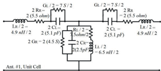
Equivalent circuit of the unit cell in Ant.#1
