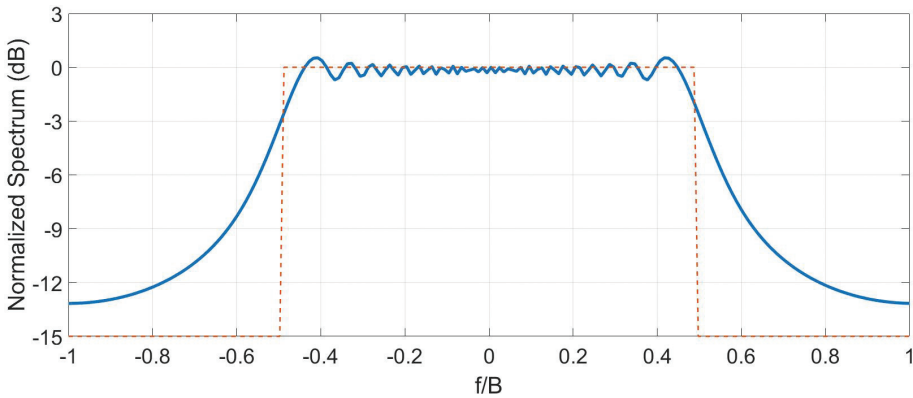
Figure 3. Normalized spectrum of a LFM signal for BT = 100 . With BT increasing, the spectrum shape is closer and closer to a rectangle (dashed line).
