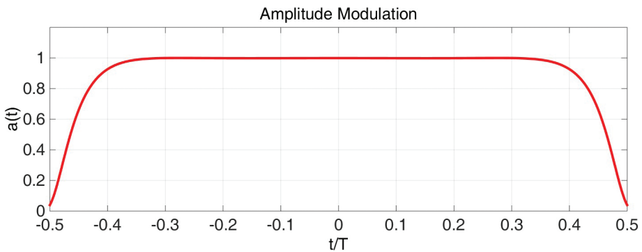
Figure 6. Optimum amplitude modulation for the HNLFM signal.
