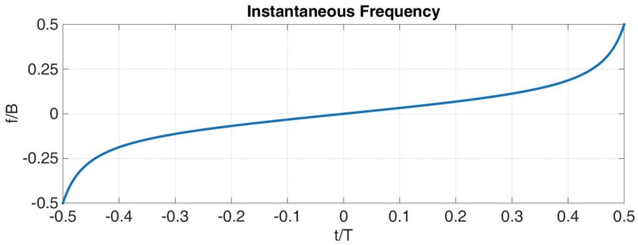
Figure 8. Instantaneous frequency of the HNLFM signal.
