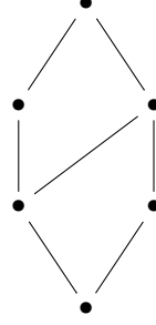
FIGURE 1. Hasse diagram of the intervals [(1, 3), (-2, 1)]^{(n-2)} and [(2, 4), (-1, 3)]^{(n-2)} .
