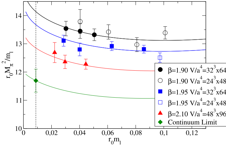
Fig. 1. Chiral and continuum extrapolation of r_0 M_\pi^2/m_\ell based on the NLO ChPT fit given by Eq. (16). Lattice data have been corrected for FSE using the CWW approach [22] and correspond to the RCs Z_P calculated with the method M1 (see text).
