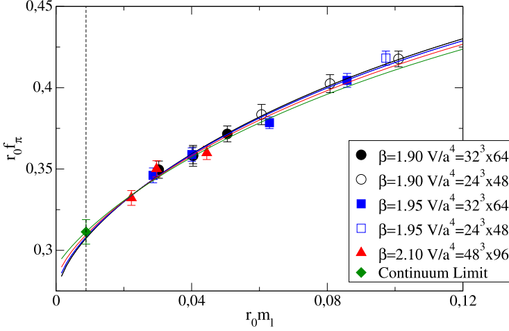
Fig. 2. The same as in Fig. 1, but for the decay constant r_0 f_\pi .
