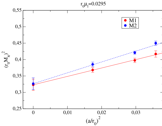
Fig. 21. Scaling of the squared pion mass computed at a fixed value of the renormalized light quark mass. The M1 and M2 determinations for Z_P lead to compatible results in the continuum limit.
