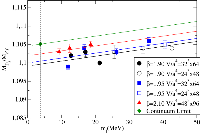
Fig. 14. Chiral and continuum extrapolations of M_{D_s}/M_{c's'} performing a linear fit in m_\ell , i.e. with \bar{P}_2 = 0 in Eq. (58).
