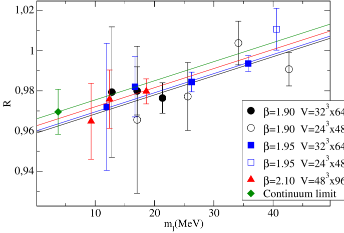
Fig. 11. Chiral and continuum extrapolations of the quantity R(m_s, m_\ell, a^2) , defined in Eq. (51), through a linear fit in m_\ell . The data are interpolated at the physical strange mass (35) and corrected for FSE.
