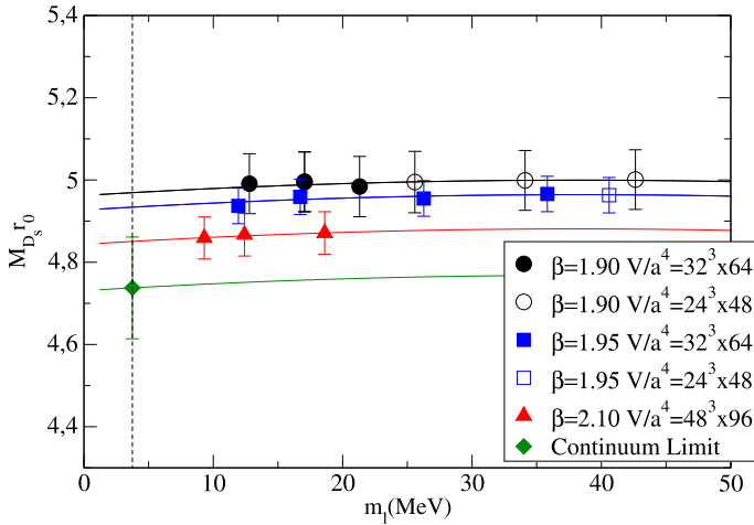
Fig. 13. The same as in Fig. 12, but in case of the quadratic fit of Eq. (56).
