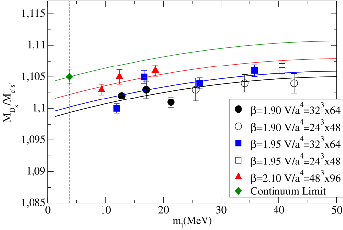
Fig. 15. The same as in Fig. 14, but in case of the quadratic fit of Eq. (58).
