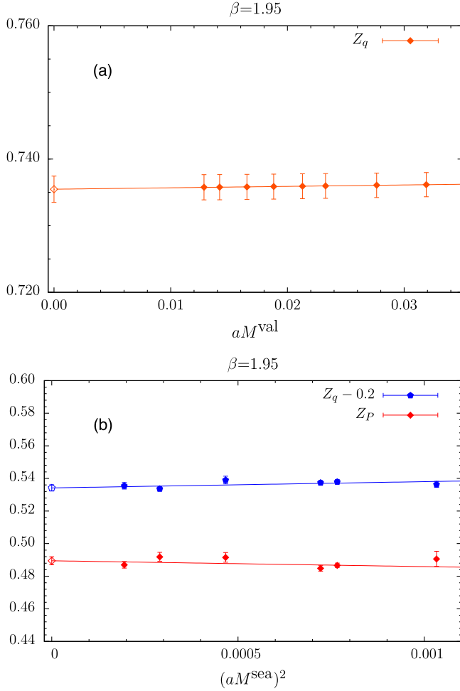
Fig. 19. Chiral extrapolations of \theta -averaged B4m and B4p data at \beta = 1.95 and (a\bar{p})^2 \approx 1.5 . Panel (a): valence quark mass extrapolation of Z_q data. Panel (b): sea quark mass extrapolation of Z_q and Z_P data. The blue dots have been displaced by 0.2 from the red squares for better visibility. (For interpretation of the references to color in this figure legend, the reader is referred to the web version of this article.)
