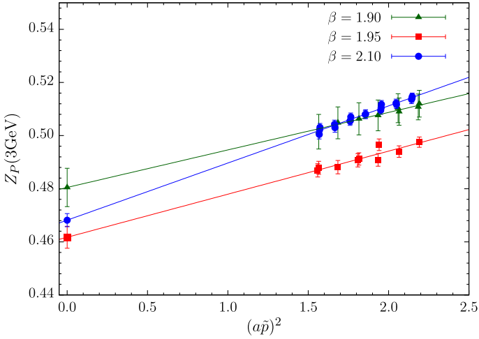
Fig. 20. Extrapolation of Z_P , obtained in the RI-MOM(3 GeV) scheme, as a function of (a\bar{p})^2 at \beta = 1.90 (green triangles), \beta = 1.95 (red squares) and \beta = 2.10 (blue dots). (For interpretation of the references to color in this figure legend, the reader is referred to the web version of this article.)
