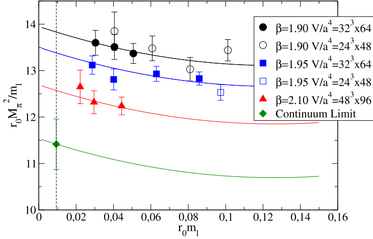
Fig. 3. Chiral and continuum extrapolation of r_0 M_\pi^2 / m_\ell obtained using the polynomial fit given by Eq. (23).
