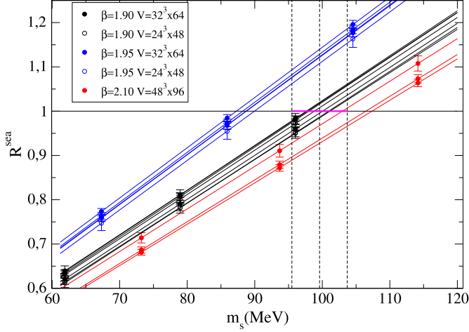
Fig. 10. The ratio R_{\text{sea}}(m_\ell, m_s, m_s^{\text{sea}}) for the various ensembles considered in this work versus the valence strange quark mass m_s . For each value of \beta and m_\ell the crossing of the interpolation curves of the lattice data with the solid line corresponding to R_{\text{sea}} = 1 identifies the location of the matching mass m_s = m_s^{\text{sea}} up to lattice artifacts (see text). The vertical dashed lines correspond to the determination (35) of the physical strange quark mass.
