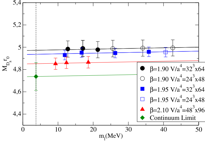
Fig. 12. Chiral and continuum extrapolation of r_0 M_{D_s} , adopting a linear fit in m_\ell , i.e. with P'_2 = 0 in Eq. (56).
