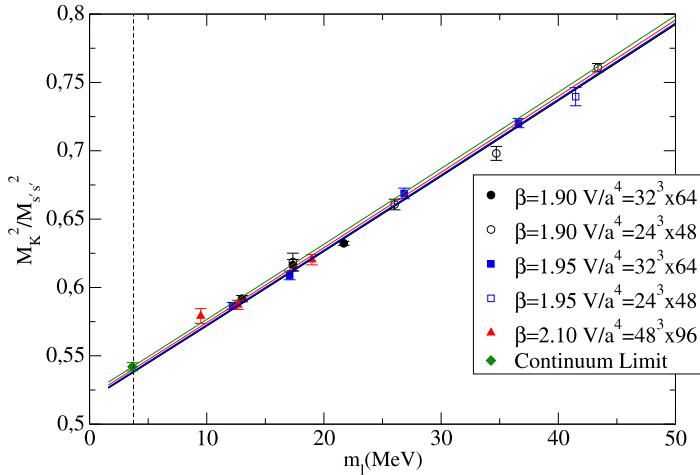
Fig. 9. Chiral and continuum extrapolation of M_K^2 in units of M_{s's'}^2 using SU(2) ChPT at NLO.
