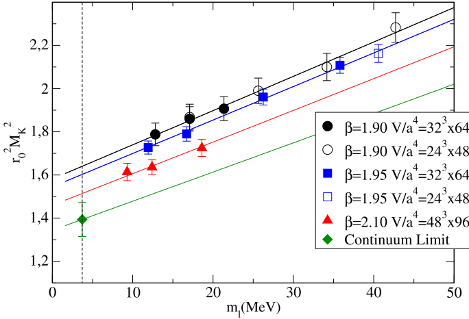
Fig. 7. Chiral and continuum extrapolation of M_K^2 in units of r_0 using the SU(2) ChPT predictions given by Eq. (33).
