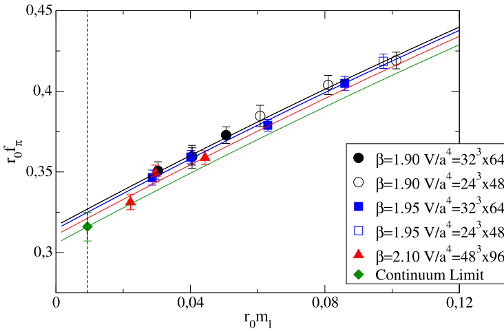
Fig. 4. The same as in Fig. 3, but for the decay constant r_0 f_\pi .
