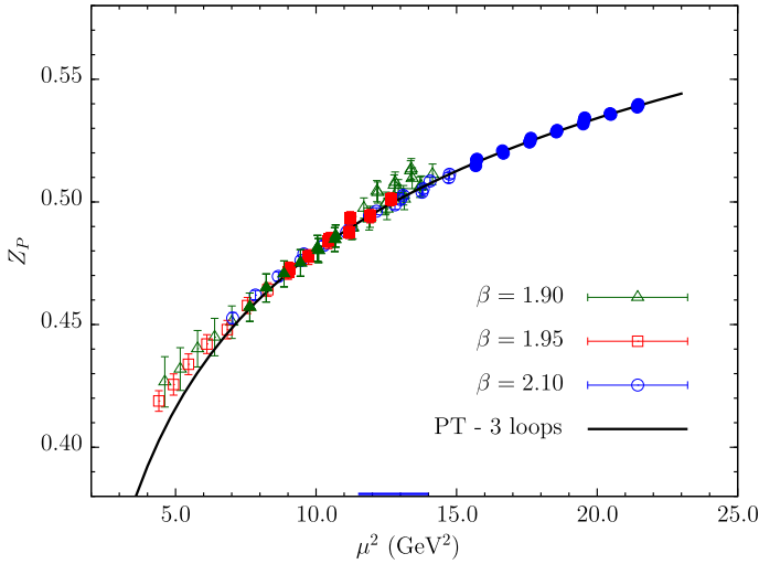
Fig. 22. Comparison of the evolution of the RC Z_P determined non-perturbatively with the one obtained in perturbation theory at three loops [62], as a function of the renormalization scale \mu . At each lattice coupling the full markers correspond to momenta (a\vec{p})^2 in the range [1.5, 2.2] used in the method M1, whereas the blue line on the x -axis identifies the range of the momenta [11.5, 14.0] \text{GeV}^2 adopted in the method M2.
