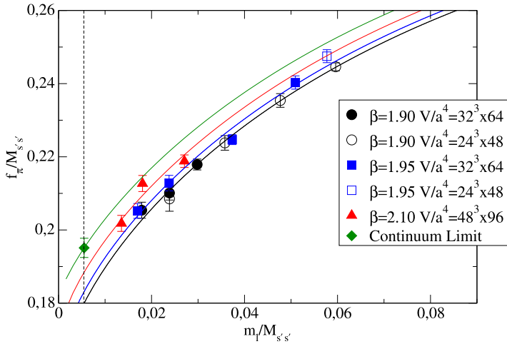
Fig. 6. The same as in Fig. 5, but for the pion decay constant f_\pi in units of M_{s's'} .
