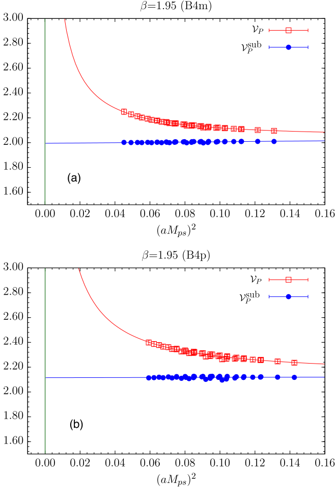
Fig. 18. Amputated pseudoscalar density two-point correlators before ( \mathcal{V}_P , red squares) and after ( \mathcal{V}_P^{\text{sub}} , blue dots) the Goldstone pole subtraction, at \beta = 1.95 and (a\tilde{p})^2 \approx 1.5 . Panels (a) and (b) correspond to data from ensembles B4m and B4p, respectively. (For interpretation of the references to color in this figure legend, the reader is referred to the web version of this article.)
