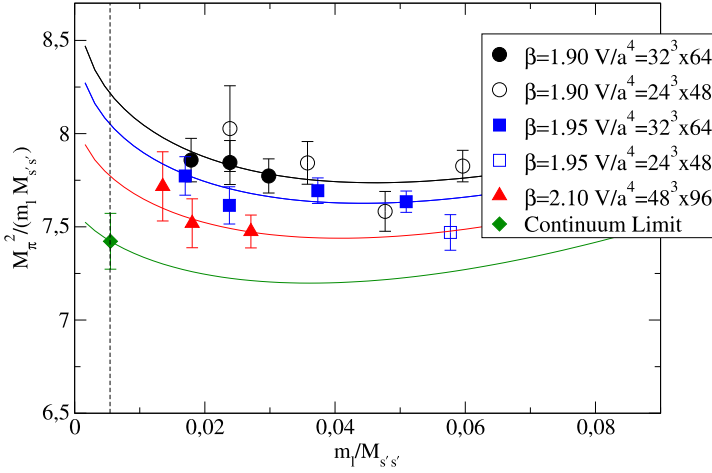
Fig. 5. Chiral and continuum extrapolation of M_\pi^2/(m_\ell M_{s's'}) obtained using the NLO ChPT fit (26).
