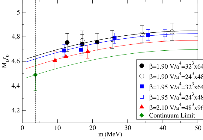
Fig. 16. Chiral and continuum extrapolations of r_0 M_D performing a quadratic fit in m_\ell .
