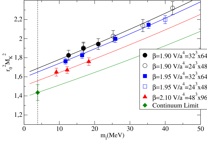
Fig. 8. The same as in Fig. 7, but in the case of the polynomial fit (34).
