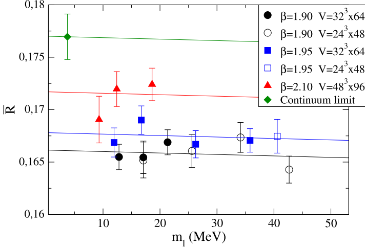
Fig. 17. Chiral and continuum extrapolations of \bar{R}(m_c, m_s, m_\ell, a^2) , defined in Eq. (63), using a linear fit in m_\ell . The data are interpolated at the physical strange and charm quark masses.
