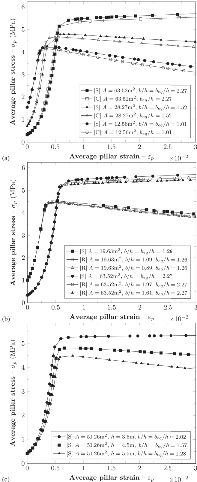
Fig. 5 Comparison of global responses: a) three couples of square and cylindrical (axi-symmetric) pillars; b) two triplets of square and rectangular pillars having the same cross-section area and ratio of the sides b/l = 0.5 and 0.75 ; c) three pillars having equal area and height h variable in the range between 3.5 and 5.5 m.
