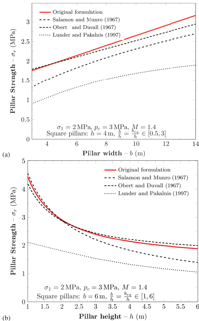
Fig. 11 Comparison of pillar strengths from proposed original formulation and three well-known formulations: a) h = 4 m is fixed and b varies in the range between 3 and 14 m; b) b = 6 m is fixed and h ranges between 1 and 6 m.
