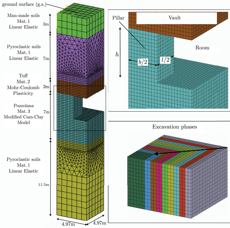
Fig. 2 Representative finite element model and definition of FE groups to be removed in order to simulate excavation for consecutive rows.
