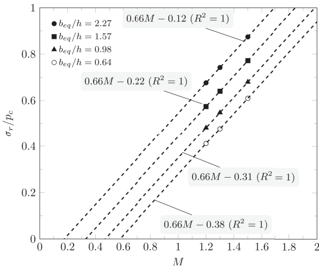
Fig. 9 Pillar strength to preconsolidation pressure \sigma_r/p_c ratio plotted against M for four values of average width-to-height ratio b_{eq}/h .
