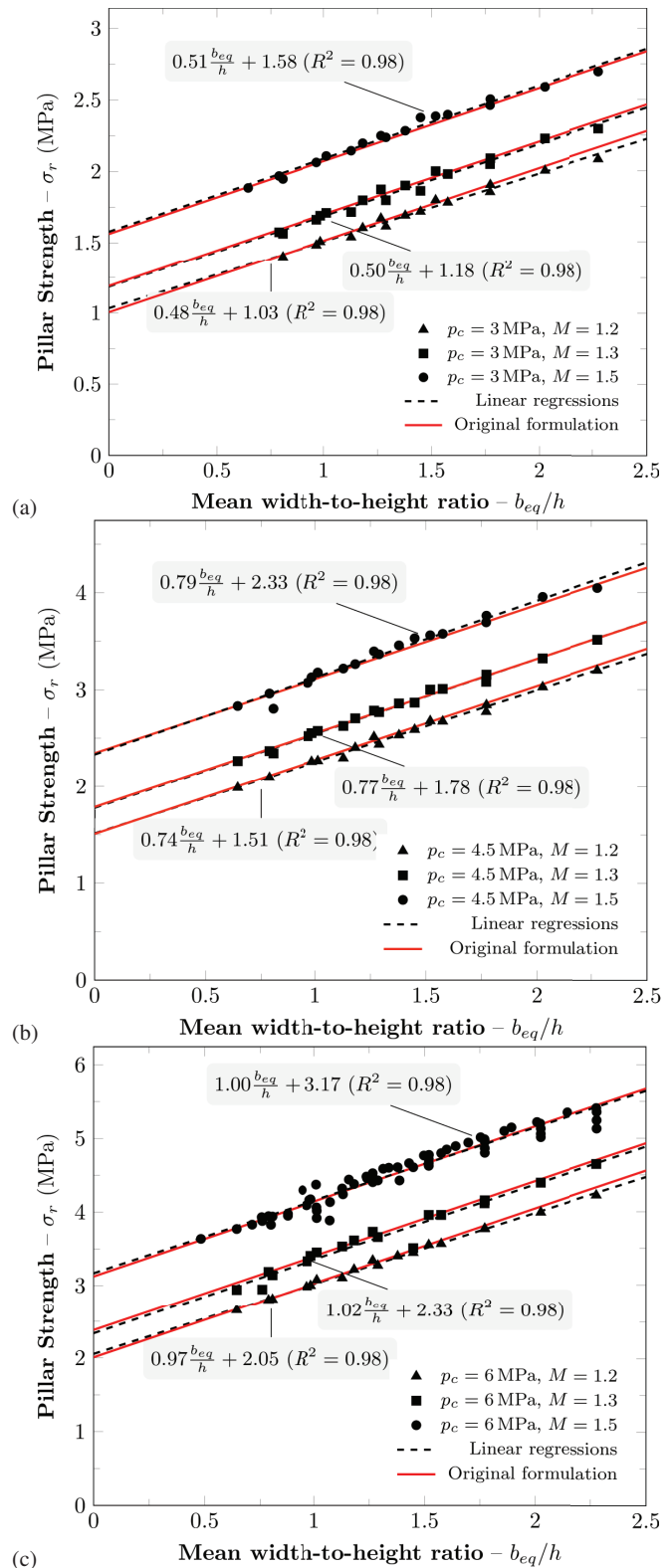
Fig. 10 Pillar strength evolution in function of average pillar width-to-height ratio and comparison with values predicted by the proposed original formulation (17).
