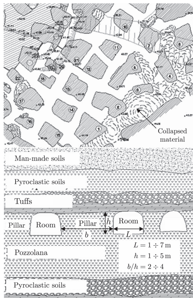
Fig. 1 Typical geometry of geotechnical system: representative plan of system of shallow cavities found in Roman subsoil.
