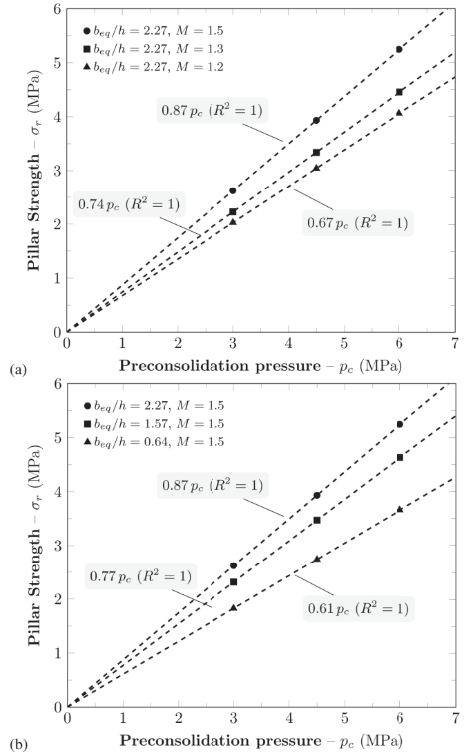
Fig. 8 Evolution of \sigma_r with respect to preconsolidation pressure p_c : a) for fixed value of average width-to-height ratio b_{eq}/h and three values of M ; b) for fixed M and three values of b_{eq}/h .
