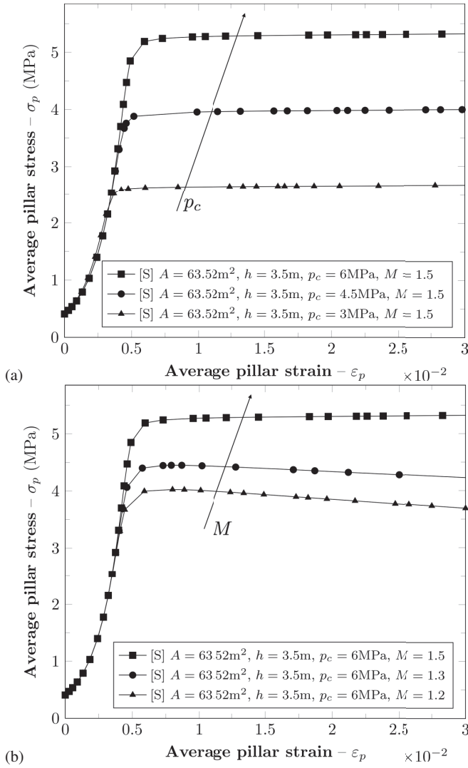
Fig. 7 Influence of p_c and M on the global response of a representative square pillar ( A = 63.52 \text{ m}^2 , h = 3.5 \text{ m} ): a) p_c is variable and M is fixed; b) p_c is fixed and M is variable.
