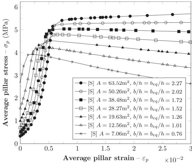
Fig. 3 Global responses of square section pillars with constant height ( h = 3.5 m) and cross-section area of 7.1 - 63.6 \text{ m}^2 .
