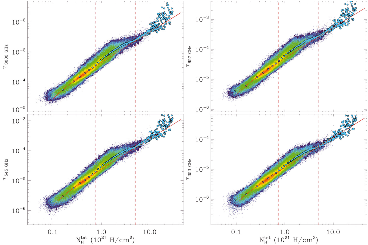
Fig. 6. Correlation plots between the dust optical depth at IRAS 100 \mu\text{m} ( upper left ), HFI 857 GHz ( upper right ), 545 GHz ( lower left ) and 353 GHz ( lower right ) and the total gas column density N_{\text{H}}^{\text{obs}} in the solar neighbourhood ( |b_{\text{II}}| > 10^\circ ). The color scale represents the density of sky pixels on a log scale. The blue dots show a N_{\text{H}}^{\text{obs}} -binned average representation of the correlation. The red line shows the best linear correlation derived at low N_{\text{H}}^{\text{obs}} values ( \tau = \left(\frac{\tau_{\text{D}}}{N_{\text{H}}}\right)^{\text{ref}} * N_{\text{H}}^{\text{obs}} + \tau_0 ). The vertical lines show the positions corresponding to A_{\text{V}} = 0.37 mag and A_{\text{V}} = 2.5 mag. These figures are shown for a single X_{\text{CO}} = 2.3 \times 10^{20} \text{ H}_2 \text{ cm}^{-2}/(\text{K km s}^{-1}) .
