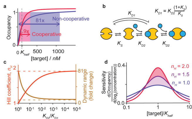
Figure 1. a) Allosteric (“Hill-type”) cooperativity provides a means of overcoming the 81-fold dynamic range of single-site receptors (blue) to produce steeper, more responsive behavior (red). Cooperativity arises when multiple binding sites interact such that the first binding event improves the affinity of subsequent binding events. b) To design this we employ the population-shift mechanism, in which the first binding event is coupled to an unfavorable conformational change, reducing its affinity ( K_{D1} ) relative to that of the second binding event ( K_{D2} ). c) While maximal cooperativity (dashed lines) is only achieved if the second binding event is infinitely more favorable than the first, near-ideal behavior is rapidly approached as the relative affinity of the subsequent binding event rises. d) Even modest cooperativity significantly improves sensitivity to small changes in concentration (shown here as the relative change in occupancy per two-fold change in target concentration).
