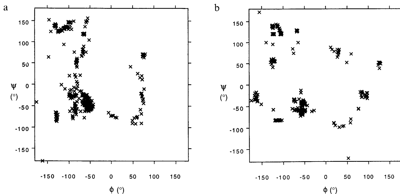
Fig. 8. Cumulative Ramachandran plot for CP1 (a) and CP1m (b) of all the 20 structures selected after restrained energy minimization.
