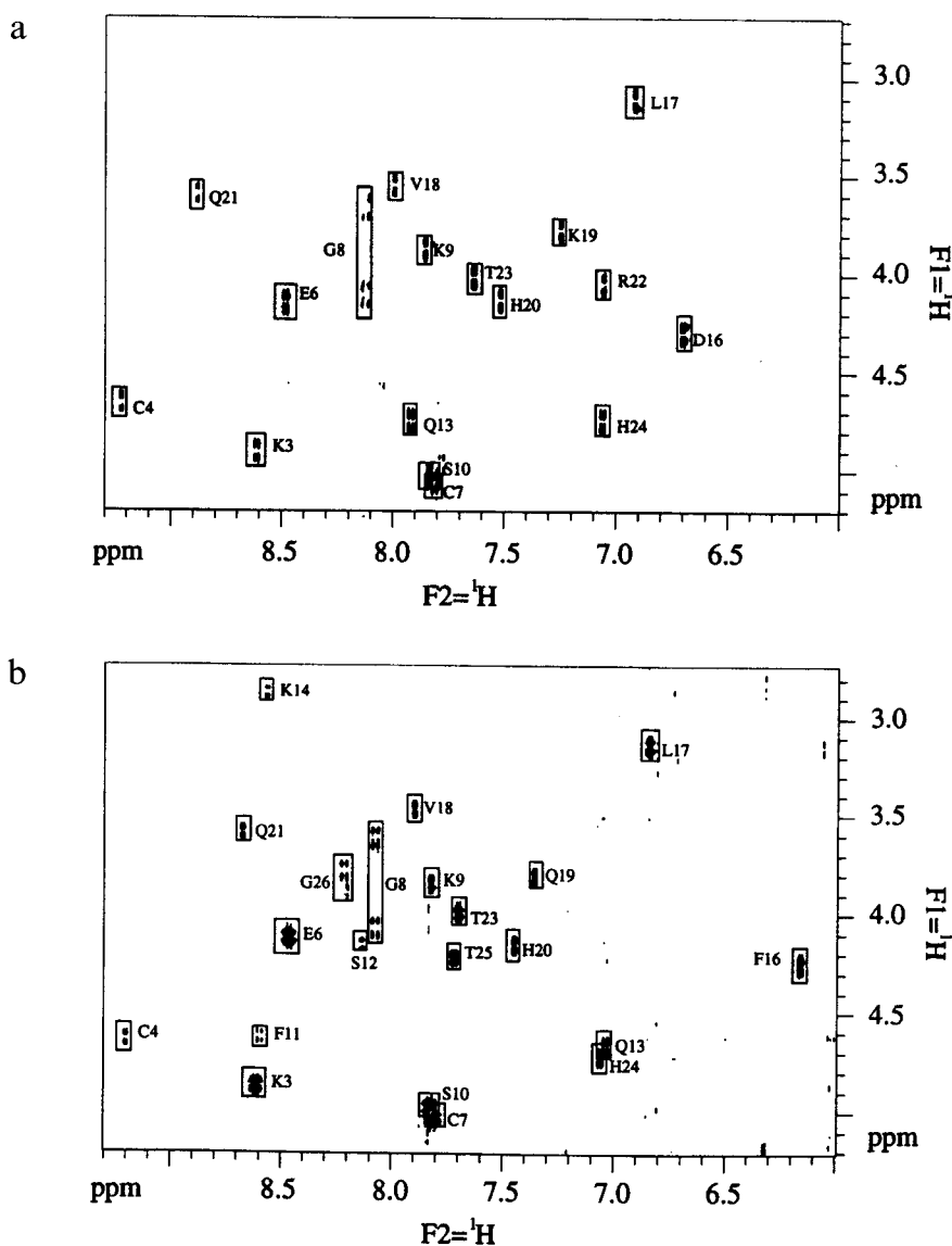
Fig. 1. Finger-print region of the COSY experiment for the CP1 (a) and CP1m (b) molecules. Signal assignment is indicated.
