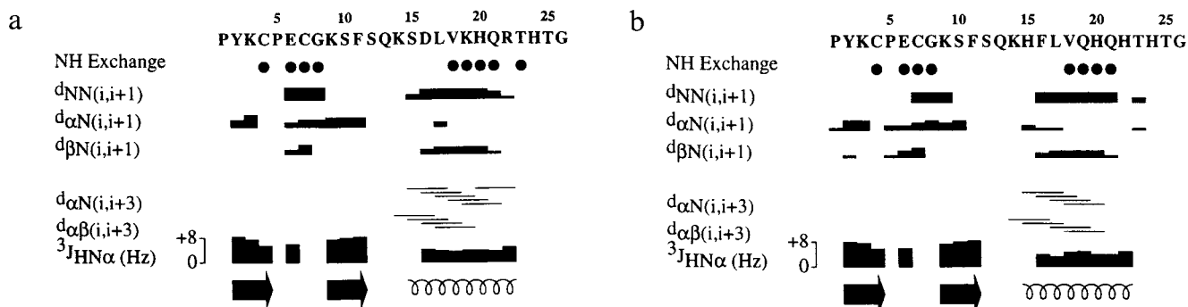
Fig. 3. Schematic representation for CPI (a) and CP1m (b) of: (i,i+1) and (i,i+3) NOEs, amide proton exchange rates and ^3J_{\text{HN}\alpha} coupling constants. The characterization of the secondary structure elements is reported at the bottom of the figure as arrows ( \beta -strands) and \alpha -helices.
