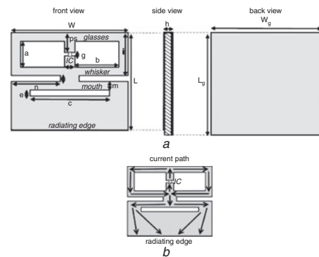
Fig. 1 Layout of miniaturised wearable tag on 3 mm-thick EPDM foam (external size: L_g = 35\text{mm} , W_g = 45\text{mm} , h = 3\text{mm} )
