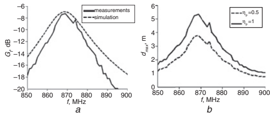
Fig. 4 Measured and simulated realised gain of miniaturised wearable tag in frontal (broadside) direction (Fig. 4a), and estimated maximum read range in free-space for case of reader with circular and linear polarisation (Fig. 4b)
