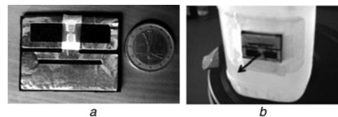
Fig. 3 RFID miniaturised wearable aluminum prototype, over 3mm EPDM black foam having dimensions as reported in Fig. 2 and mouth and whisker parameters c = 29\text{mm} , n = 18\text{mm}
