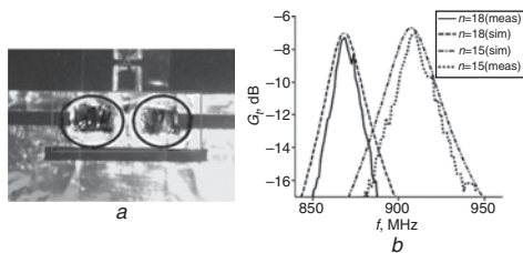
Fig. 5 Wearable prototype with additional strips of aluminium to shorten 'n' from 18 to 15 mm (Fig. 5a), and measured and simulated realised gain for tag in frontal (broadside) direction with n equal to 18 and 15 mm (Fig. 5b)
