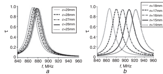
Fig. 2 Parametric exploration of simulated power transmission coefficient for various lengths
