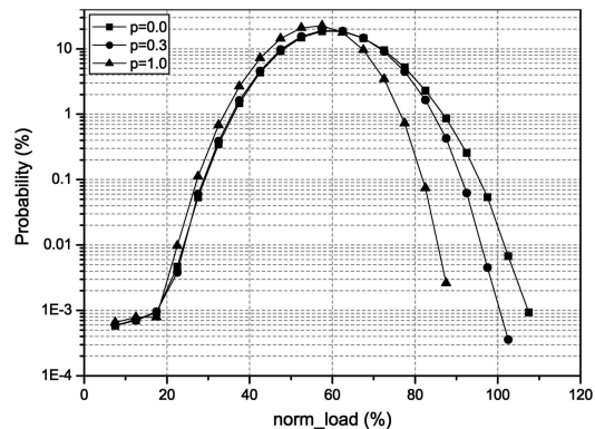
Fig. 18. PDF of norm_load for TCP_perc = 100, L = 9000 kbit/s, mob_ratio = 1, BPR_1 = BPR_2 = 1 .
