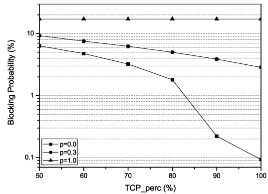
Fig. 15. BP versus percentage of TCP connections for different TCP\_perc values, BPR_1 = BPR_2 = 1 , mob\_ratio = 1 , L = 9000 kbit/s.
