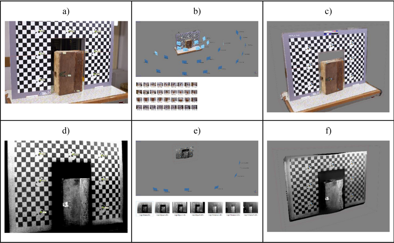
Fig. 2. Schematic view of the steps involved in the generation of the IR 3D model using the reference panel: a) automatic target recognition; b) SfM - RGB images; c) Hi res 3D Model RGB images; d) Semi-automatic target recognition; e) SfM - MWIR images; f) Low res 3D model IR calibrated images.
