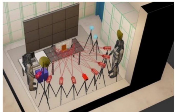
Fig. 3. Schematic representation of the MWIR Reflectography and PT images recording procedure.
