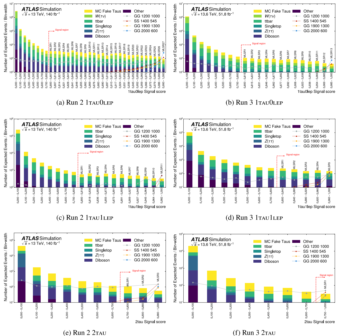
Fig. 2 Expected background composition across the range of signal scores. The numbers of events shown are normalised to their bin-width. Benchmark signal points are overlayed
