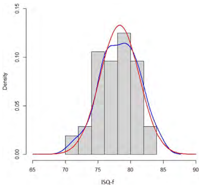
FIGURE 16 ISQ-f empirical distribution (blue line: kernel density estimate, red line: fitted normal density)
