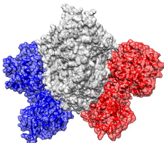
Figure 8. Comparison between the transferrin and transferrin receptor 1 (Tf-TfR1) crystallographic structures (PDB ID: 3S9L) and the obtained human lactoferrin (hLf)-TfR1 docking pose. Both TfR1 monomers are represented in grey; Tf is represented by a blue transparent surface bound to TfR1 monomer A, while hLf is in red bound on TfR1 monomer B. Both TfR1 monomers are equivalent for sequence, structure and interactions, Tf and hLf can therefore occupy the same location.
