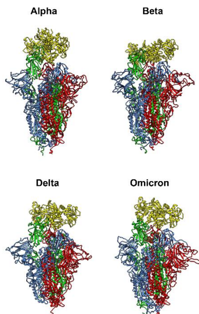
Figure 10. Complex between bovine lactoferrin (bLf) and the four Spike variants of interest obtained through molecular docking simulations. bLf is represented with yellow ribbons, while the three different chains composing the Spike glycoprotein are represented by red, blue, and green ribbons.
