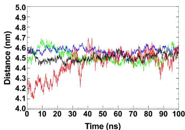
Figure 11. Time-dependent analysis of the distance evaluated between the centers of mass of the bovine lactoferrin and the receptor binding domain in the up conformation of the four Spike variants (black: Alpha, red: Beta, green: Delta and blue: Omicron).
