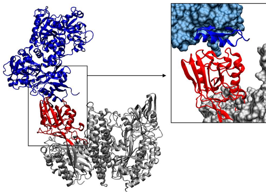
Figure 9. Complex obtained between bovine lactoferrin (bLf) (in blue) and human transferrin receptor 1 (TfR1) (in grey). The apical domain of TfR1, binding site of bLf, is highlighted in red. A closer representation of the interaction site is shown in the right image, where the proteins are represented as a solid surface, except for the interacting regions that are shown as cartoons.
