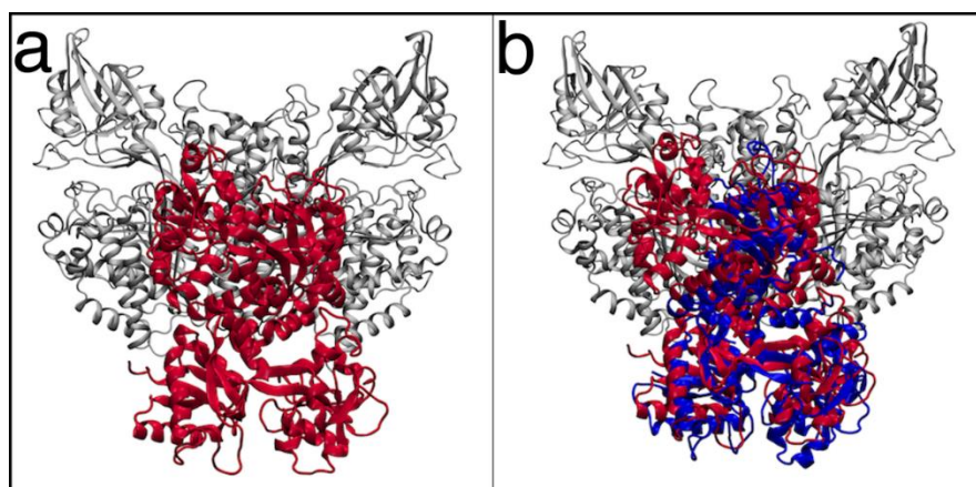
Figure 7. (a) Complex between human lactoferrin (hLf) (in red) and transferrin receptor 1 (TfR1) (in grey) obtained through molecular docking simulations. (b) Superposition of the hLf-TfR1 docking pose with the Tf-TfR1 crystallographic structure (PDB ID: 3S9L).
