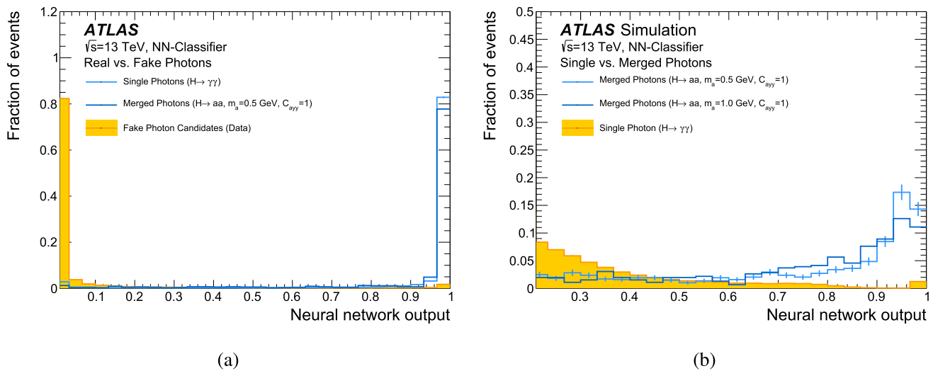
Fig. 1 Output of the neural network classifier to distinguish a real from fake photons, and b single from merged photons
