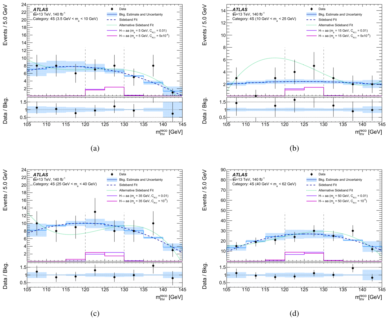
Fig. 3 m_{inv}^{reco} distribution for the nominal signal selection for the 4S category. The nominal sideband fitting function is shown as the blue dashed line. The background, estimated from a fit in the side-band regions, and its systematic variation (obtained from a fit with reduced range) is shown as the blue histogram. The green dotted line shows the alternative fitting function which is used to estimate the spurious signal uncertainty (discussed in Sect. 6). The four subfigures show different ALP mass ranges: a 3.5 \text{ GeV} < m_a < 10 \text{ GeV} , b 10 \text{ GeV} < m_a < 25 \text{ GeV} , c 25 \text{ GeV} < m_a < 40 \text{ GeV} , d 40 \text{ GeV} < m_a < 62 \text{ GeV} . The sig-
