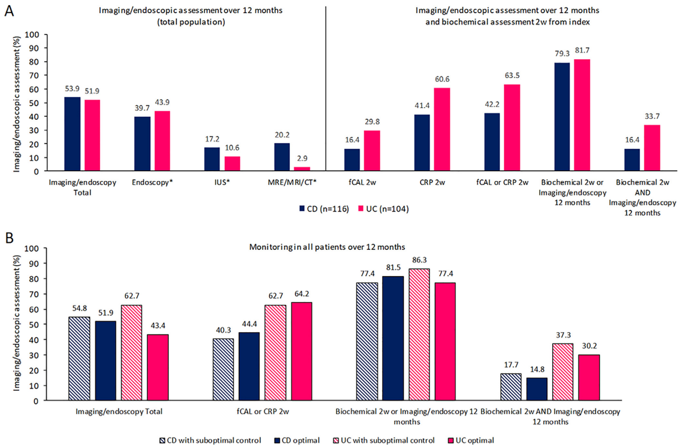
Fig. 3. Imaging/endoscopic and biochemical assessment over a period of 12 months and 2 weeks from the index date (A), and imaging/endoscopic assessment over a 12-month period for both optimally and suboptimally controlled cases of Ulcerative Colitis (UC) and Crohn's Disease (CD) (B). *More than one assessment may occur in the same patient (sum of individual assessments may not equal total).
