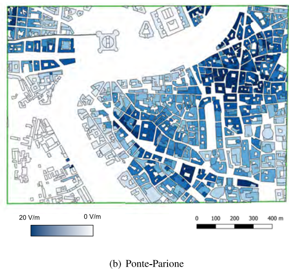
FIGURE 17. EMF exposure E_b^{TOT} over the buildings (5G maturity setting).
