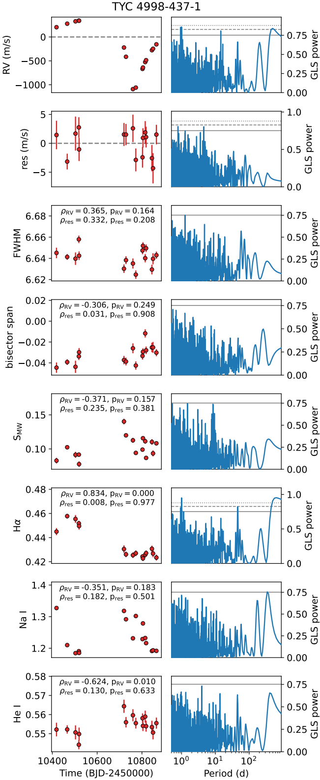
Fig. B.7. Same as Fig. B.1 but for star TYC 4998-437-1
