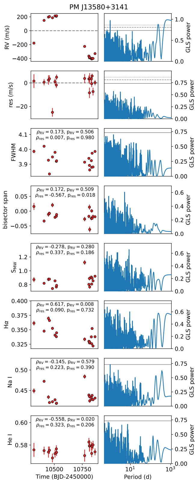
Fig. B.5. Same as Fig. B.1 but for star PM J13580+3141
