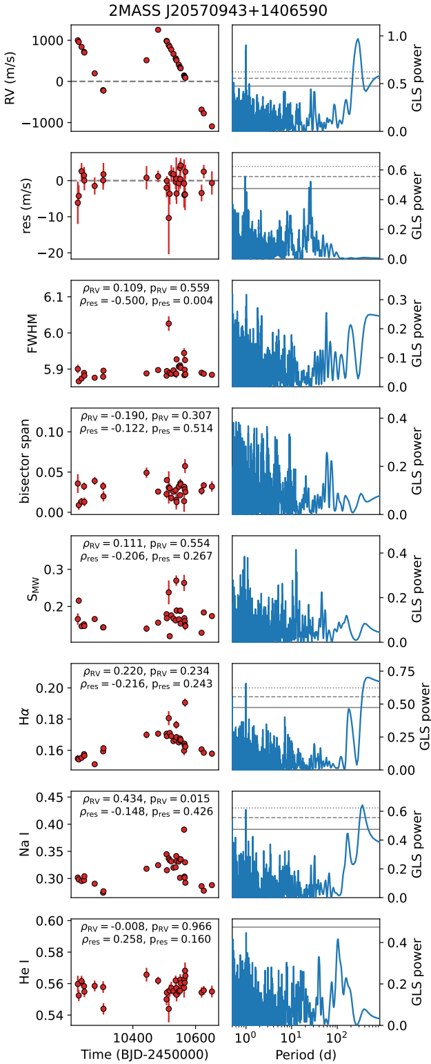
Fig. B.1. Left panels: time series for the HARPS-N median-subtracted radial velocity data of 2MASS J20570943+1406590, post-Keplerian fit residuals and activity indices. For the activity indices time series, the Pearson correlation coefficient and its p-value with both original and residual RVs are noted. Right panels: corresponding generalised Lomb-Scargle periodograms of the time series, with horizontal solid, dashed and dotted lines marking the 10%, 1% and 0.1% FAP thresholds.
