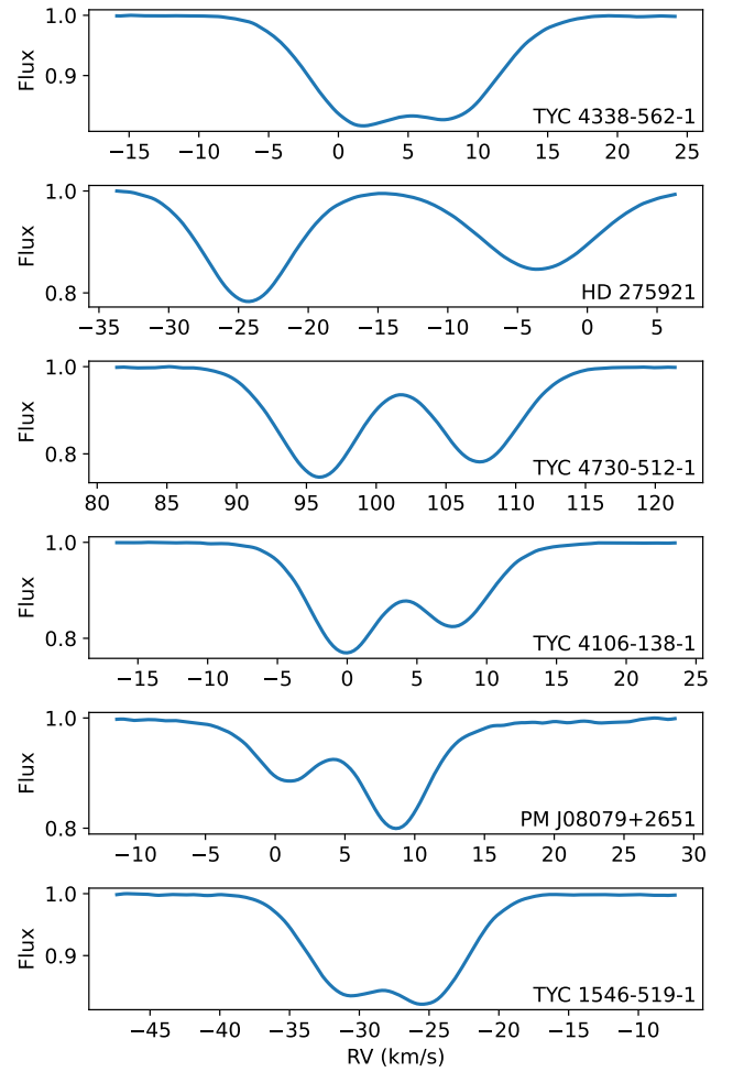
Fig. 1. HARPS-N cross correlation function profiles of the six stars in the sample identified as binaries mimicking sub-stellar astrometric motion.
