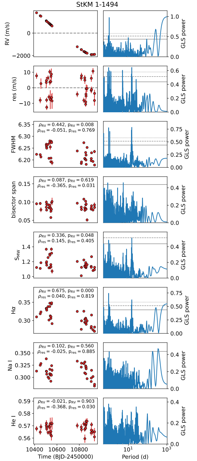
Fig. B.8. Same as Fig. B.1 but for star StKM 1-1494
