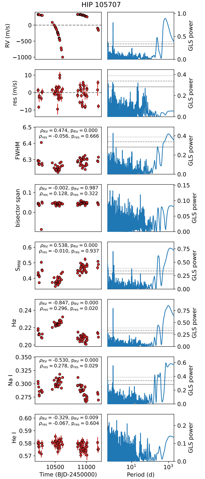
Fig. B.2. Same as Fig. B.1 but for star HIP 105707
