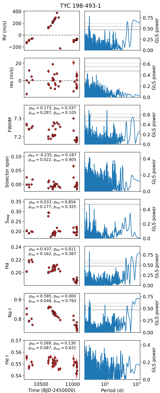
Fig. B.3. Same as Fig. B.1 but for star TYC 198-493-1
